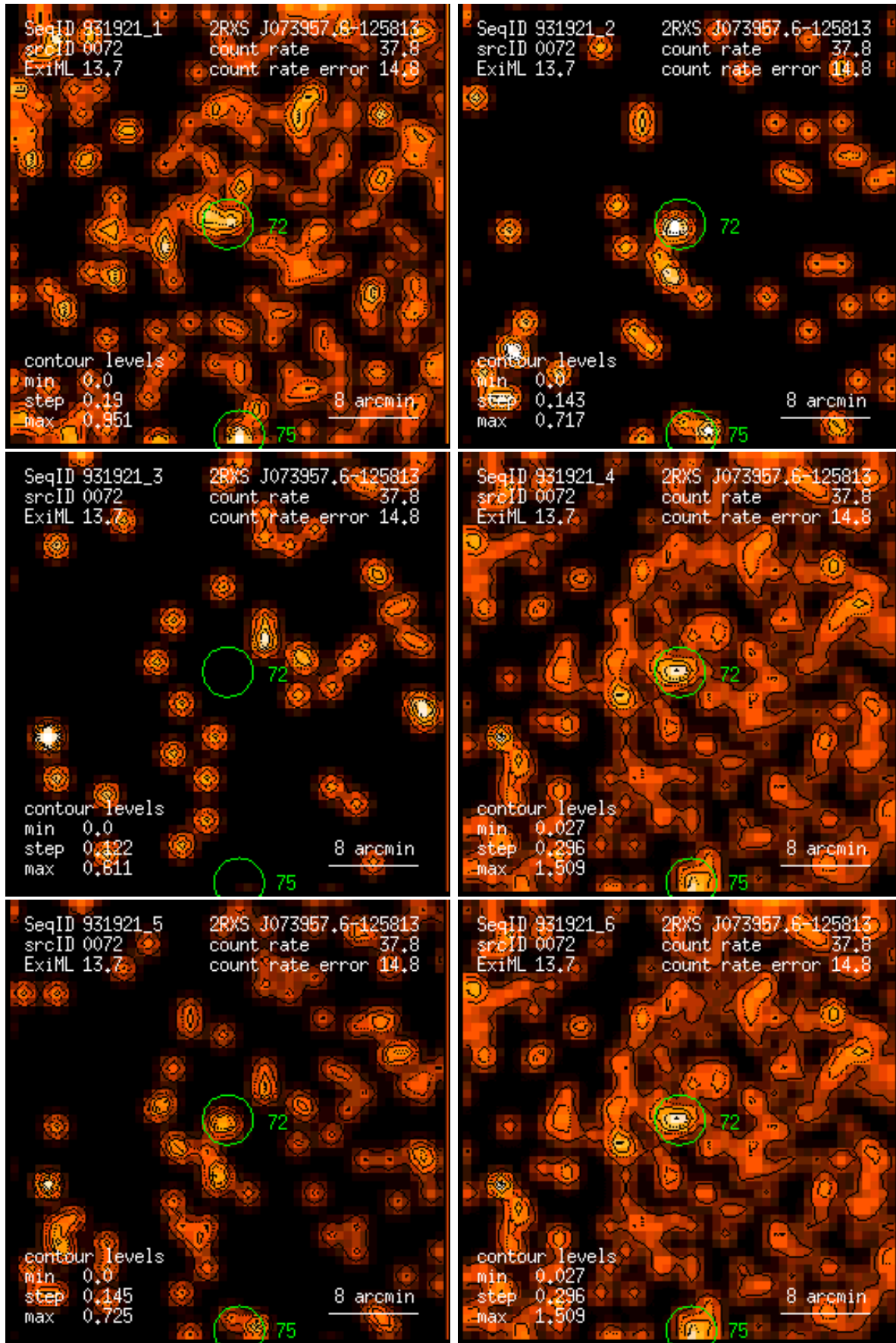
Figure 72: RASS 931921: detection 0072: band rate images, Gaussian filter: (1) PSPC channels 11 – 41, (2) 52 – 90, (3) 91 – 201, (4) 11 – 235, (5) 52 – 201, (6) 11 – 201. Broad band rates in counts/ks. Band rate contour levels in counts/ks/arcmin 2 .
