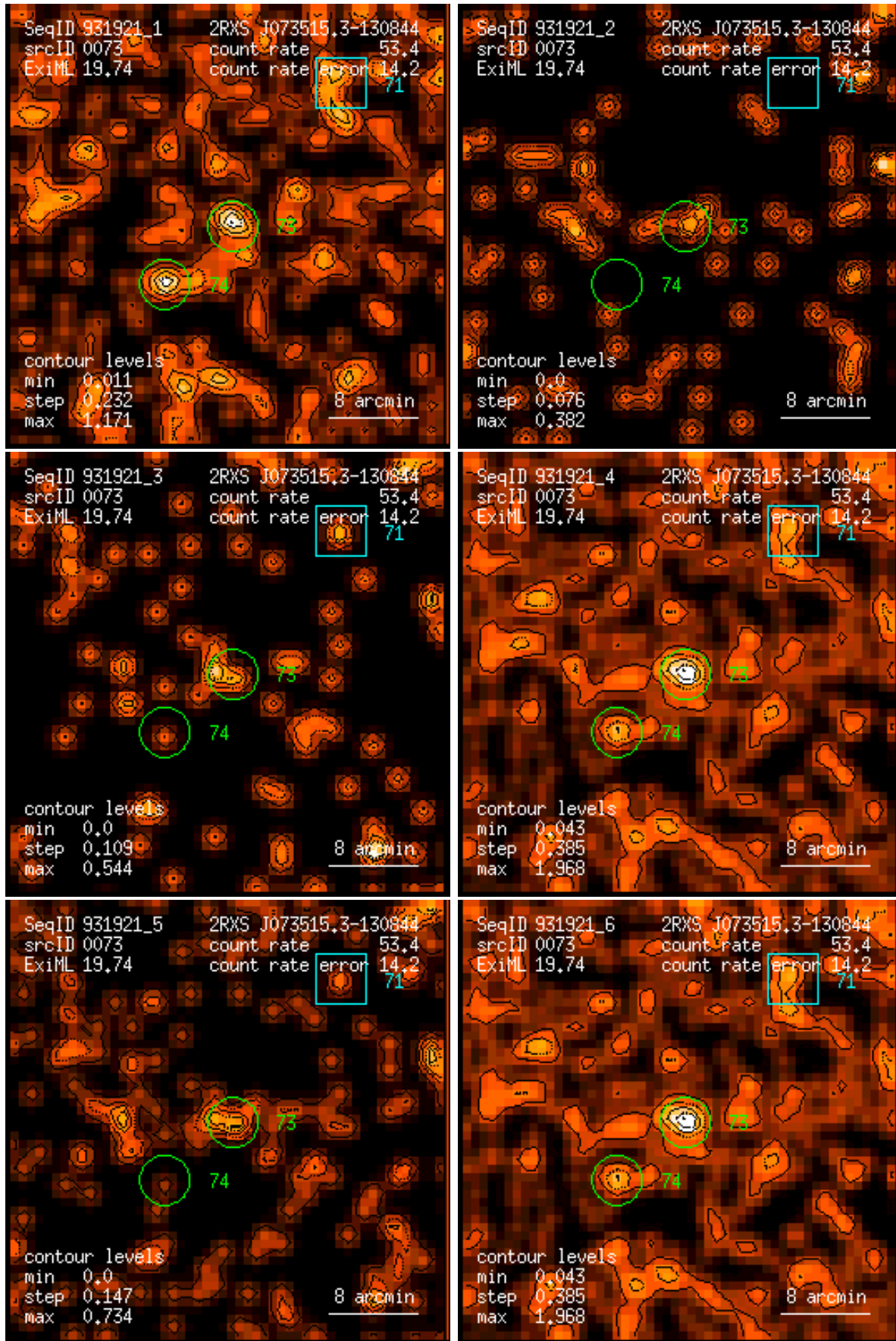
Figure 73: RASS 931921: detection 0073: band rate images, Gaussian filter: (1) PSPC channels 11 – 41, (2) 52 – 90, (3) 91 – 201, (4) 11 – 235, (5) 52 – 201, (6) 11 – 201. Broad band rates in counts/ks. Band rate contour levels in counts/ks/arcmin 2 .
