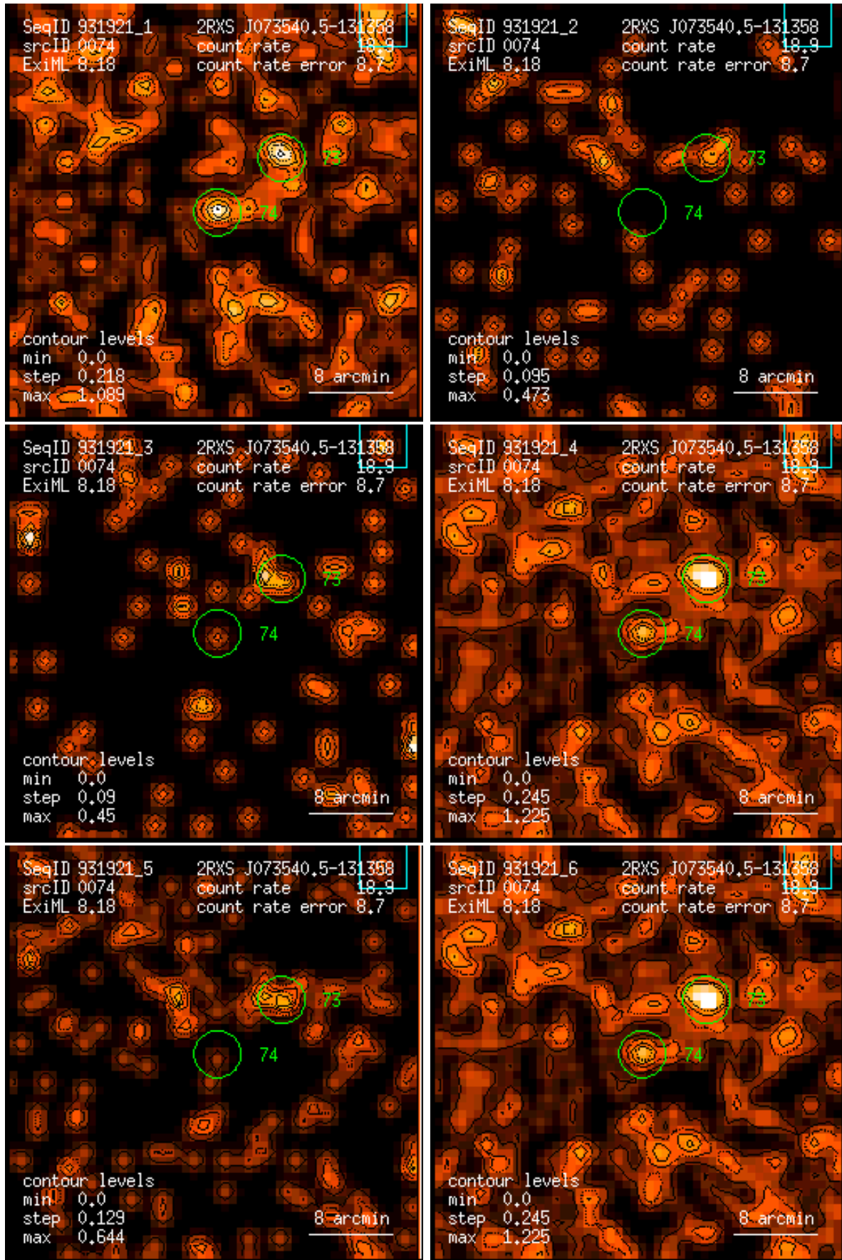
Figure 74: RASS 931921: detection 0074: band rate images, Gaussian filter: (1) PSPC channels 11 – 41, (2) 52 – 90, (3) 91 – 201, (4) 11 – 235, (5) 52 – 201, (6) 11 – 201. Broad band rates in counts/ks. Band rate contour levels in counts/ks/arcmin 2 .
