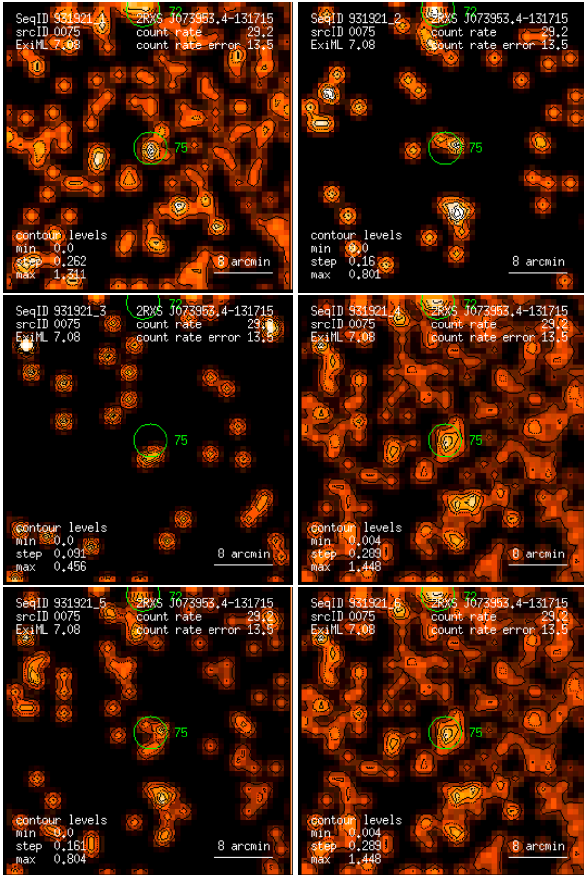
Figure 75: RASS 931921: detection 0075: band rate images, Gaussian filter: (1) PSPC channels 11 – 41, (2) 52 – 90, (3) 91 – 201, (4) 11 – 235, (5) 52 – 201, (6) 11 – 201. Broad band rates in counts/ks. Band rate contour levels in counts/ks/arcmin 2 .
