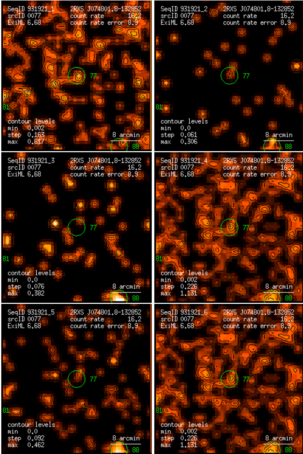
Figure 77: RASS 931921: detection 0077: band rate images, Gaussian filter: (1) PSPC channels 11 – 41, (2) 52 – 90, (3) 91 – 201, (4) 11 – 235, (5) 52 – 201, (6) 11 – 201. Broad band rates in counts/ks. Band rate contour levels in counts/ks/arcmin 2 .
