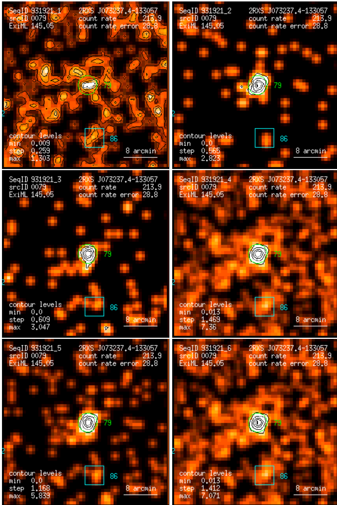
Figure 79: RASS 931921: detection 0079: band rate images, Gaussian filter: (1) PSPC channels 11 – 41, (2) 52 – 90, (3) 91 – 201, (4) 11 – 235, (5) 52 – 201, (6) 11 – 201. Broad band rates in counts/ks. Band rate contour levels in counts/ks/arcmin 2 .
