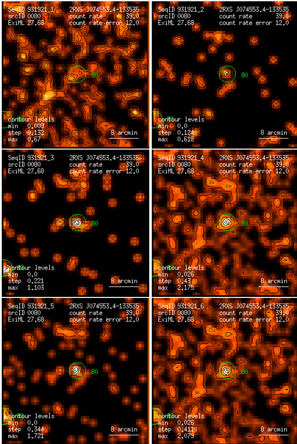
Figure 80: RASS 931921: detection 0080: band rate images, Gaussian filter: (1) PSPC channels 11 – 41, (2) 52 – 90, (3) 91 – 201, (4) 11 – 235, (5) 52 – 201, (6) 11 – 201. Broad band rates in counts/ks. Band rate contour levels in counts/ks/arcmin 2 .
