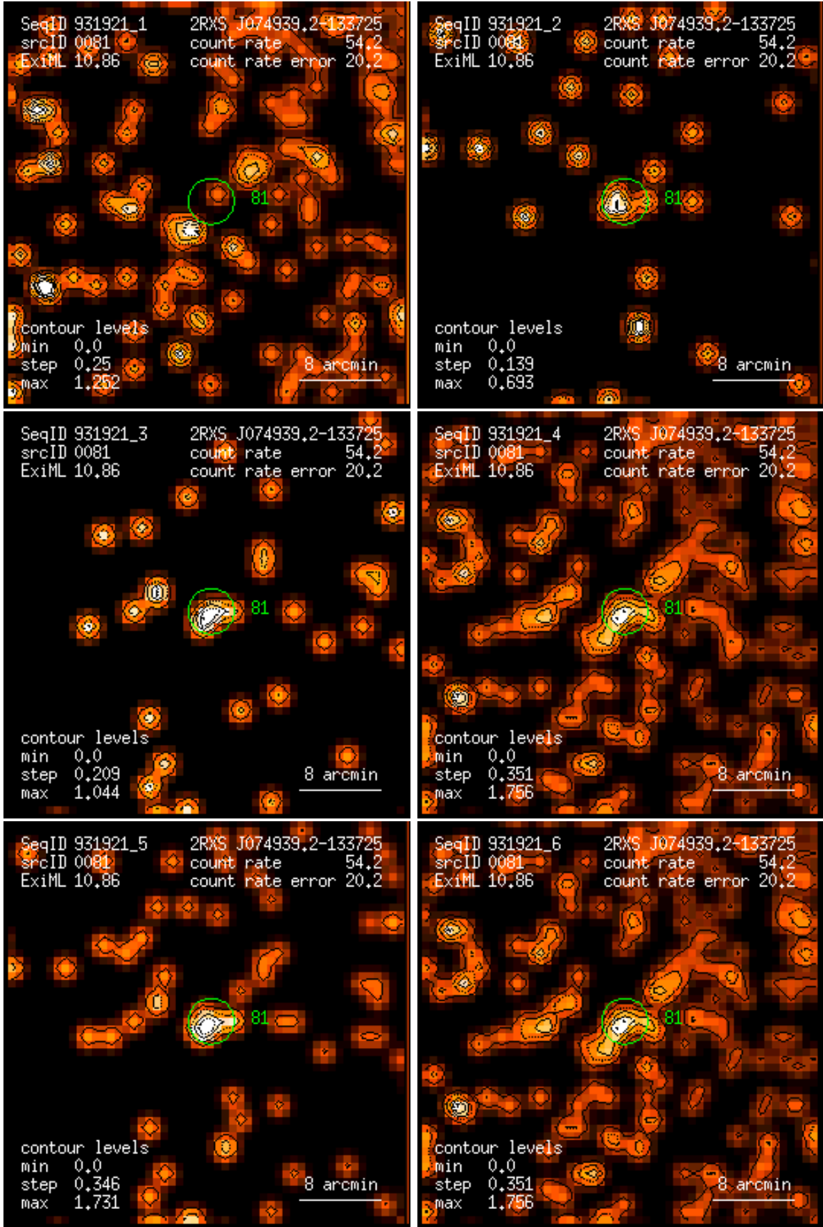
Figure 81: RASS 931921: detection 0081: band rate images, Gaussian filter: (1) PSPC channels 11 – 41, (2) 52 – 90, (3) 91 – 201, (4) 11 – 235, (5) 52 – 201, (6) 11 – 201. Broad band rates in counts/ks. Band rate contour levels in counts/ks/arcmin 2 .
