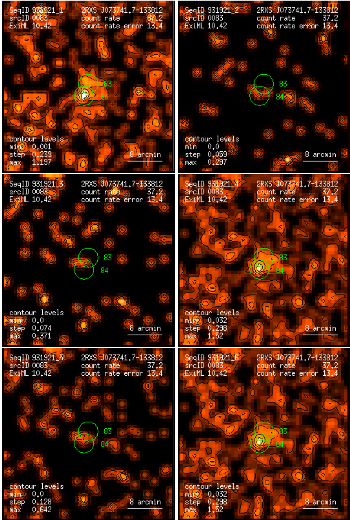
Figure 83: RASS 931921: detection 0083: band rate images, Gaussian filter: (1) PSPC channels 11 – 41, (2) 52 – 90, (3) 91 – 201, (4) 11 – 235, (5) 52 – 201, (6) 11 – 201. Broad band rates in counts/ks. Band rate contour levels in counts/ks/arcmin 2 .
