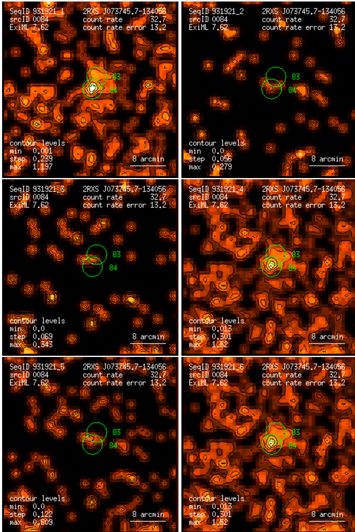
Figure 84: RASS 931921: detection 0084: band rate images, Gaussian filter: (1) PSPC channels 11 – 41, (2) 52 – 90, (3) 91 – 201, (4) 11 – 235, (5) 52 – 201, (6) 11 – 201. Broad band rates in counts/ks. Band rate contour levels in counts/ks/arcmin 2 .
