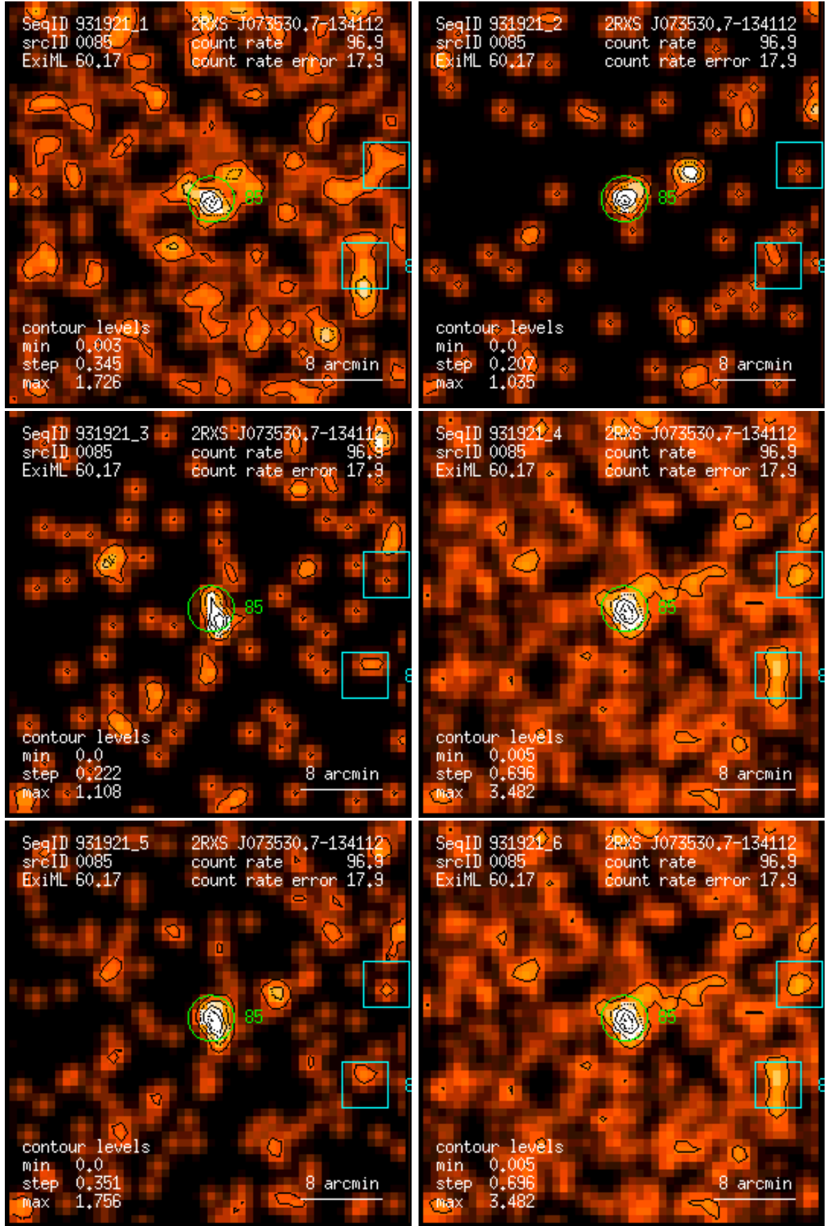
Figure 85: RASS 931921: detection 0085: band rate images, Gaussian filter: (1) PSPC channels 11 – 41, (2) 52 – 90, (3) 91 – 201, (4) 11 – 235, (5) 52 – 201, (6) 11 – 201. Broad band rates in counts/ks. Band rate contour levels in counts/ks/arcmin 2 .
