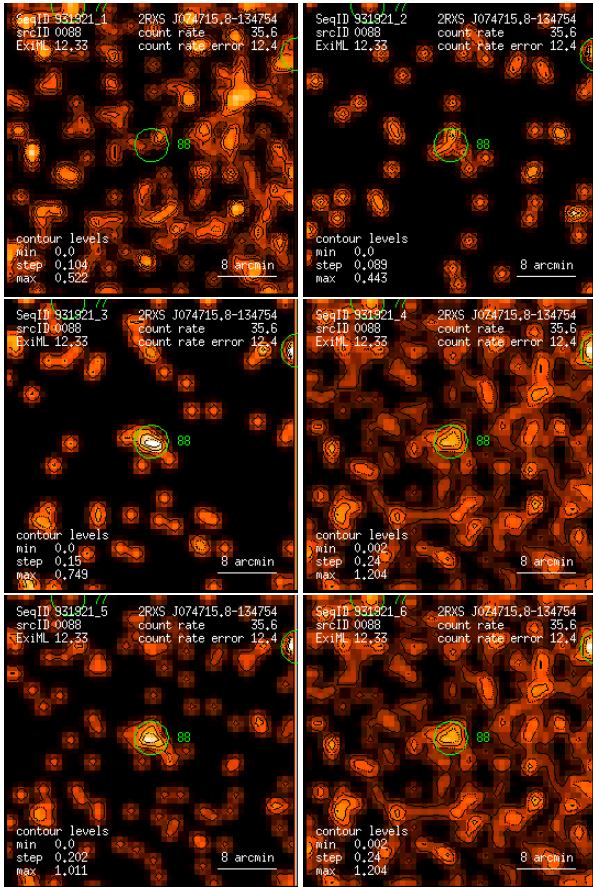
Figure 88: RASS 931921: detection 0088: band rate images, Gaussian filter: (1) PSPC channels 11 – 41, (2) 52 – 90, (3) 91 – 201, (4) 11 – 235, (5) 52 – 201, (6) 11 – 201. Broad band rates in counts/ks. Band rate contour levels in counts/ks/arcmin 2 .
