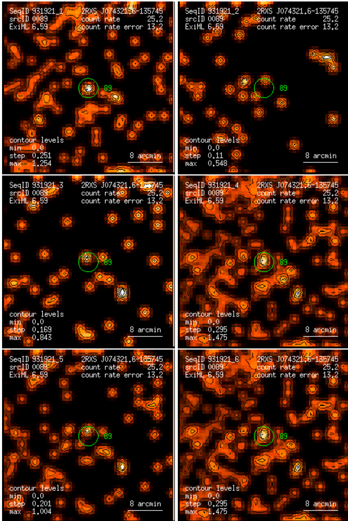
Figure 89: RASS 931921: detection 0089: band rate images, Gaussian filter: (1) PSPC channels 11 – 41, (2) 52 – 90, (3) 91 – 201, (4) 11 – 235, (5) 52 – 201, (6) 11 – 201. Broad band rates in counts/ks. Band rate contour levels in counts/ks/arcmin 2 .
