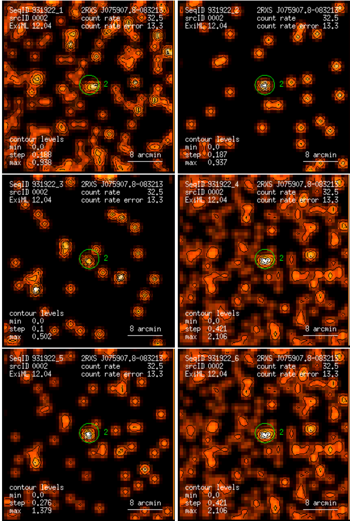
Figure 2: RASS 931922: detection 0002: band rate images, Gaussian filter: (1) PSPC channels 11 – 41, (2) 52 – 90, (3) 91 – 201, (4) 11 – 235, (5) 52 – 201, (6) 11 – 201. Broad band rates in counts/ks. Band rate contour levels in counts/ks/arcmin 2 .
