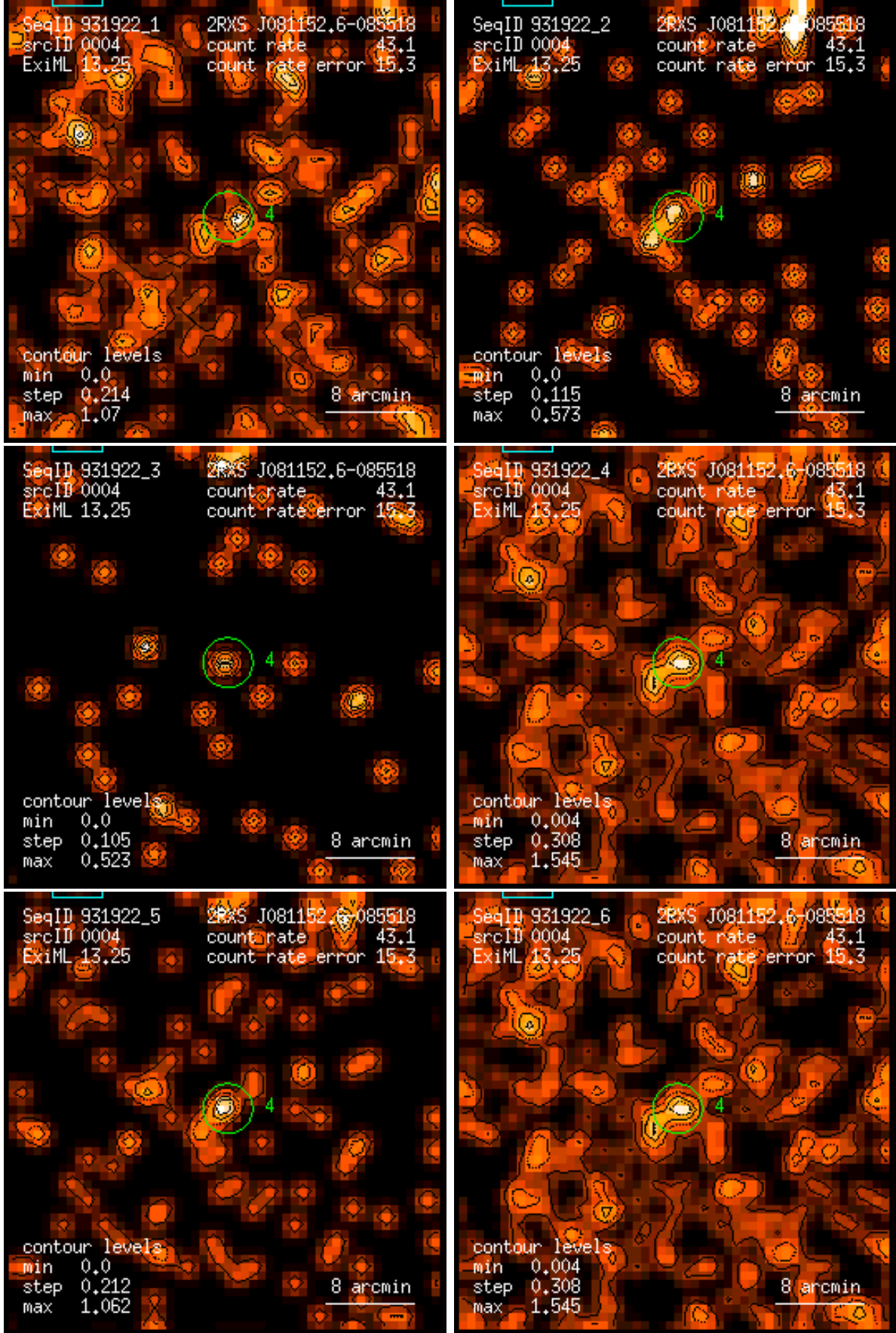
Figure 4: RASS 931922: detection 0004: band rate images, Gaussian filter: (1) PSPC channels 11 – 41, (2) 52 – 90, (3) 91 – 201, (4) 11 – 235, (5) 52 – 201, (6) 11 – 201. Broad band rates in counts/ks. Band rate contour levels in counts/ks/arcmin 2 .
