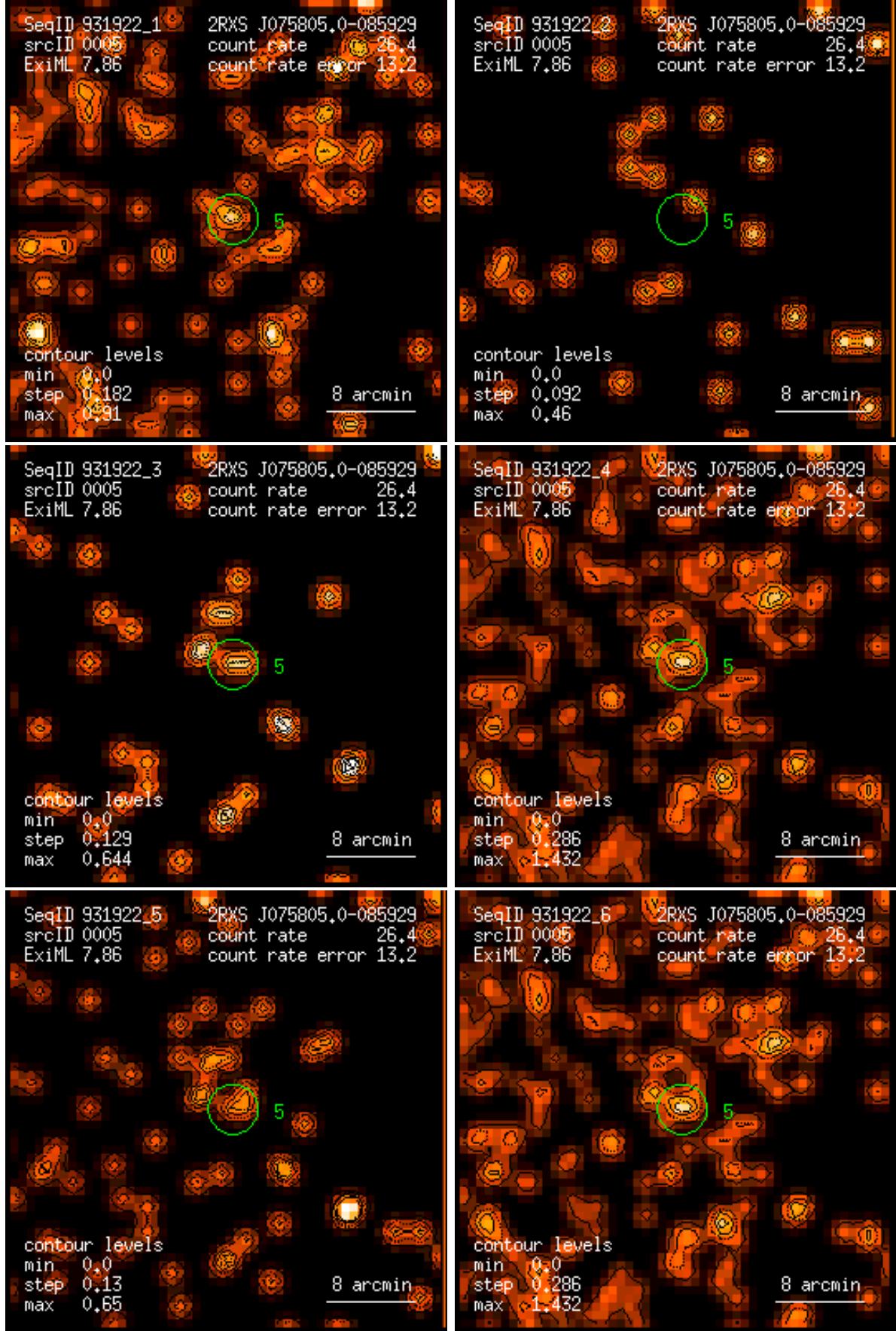
Figure 5: RASS 931922: detection 0005: band rate images, Gaussian filter: (1) PSPC channels 11 – 41, (2) 52 – 90, (3) 91 – 201, (4) 11 – 235, (5) 52 – 201, (6) 11 – 201. Broad band rates in counts/ks. Band rate contour levels in counts/ks/arcmin 2 .
