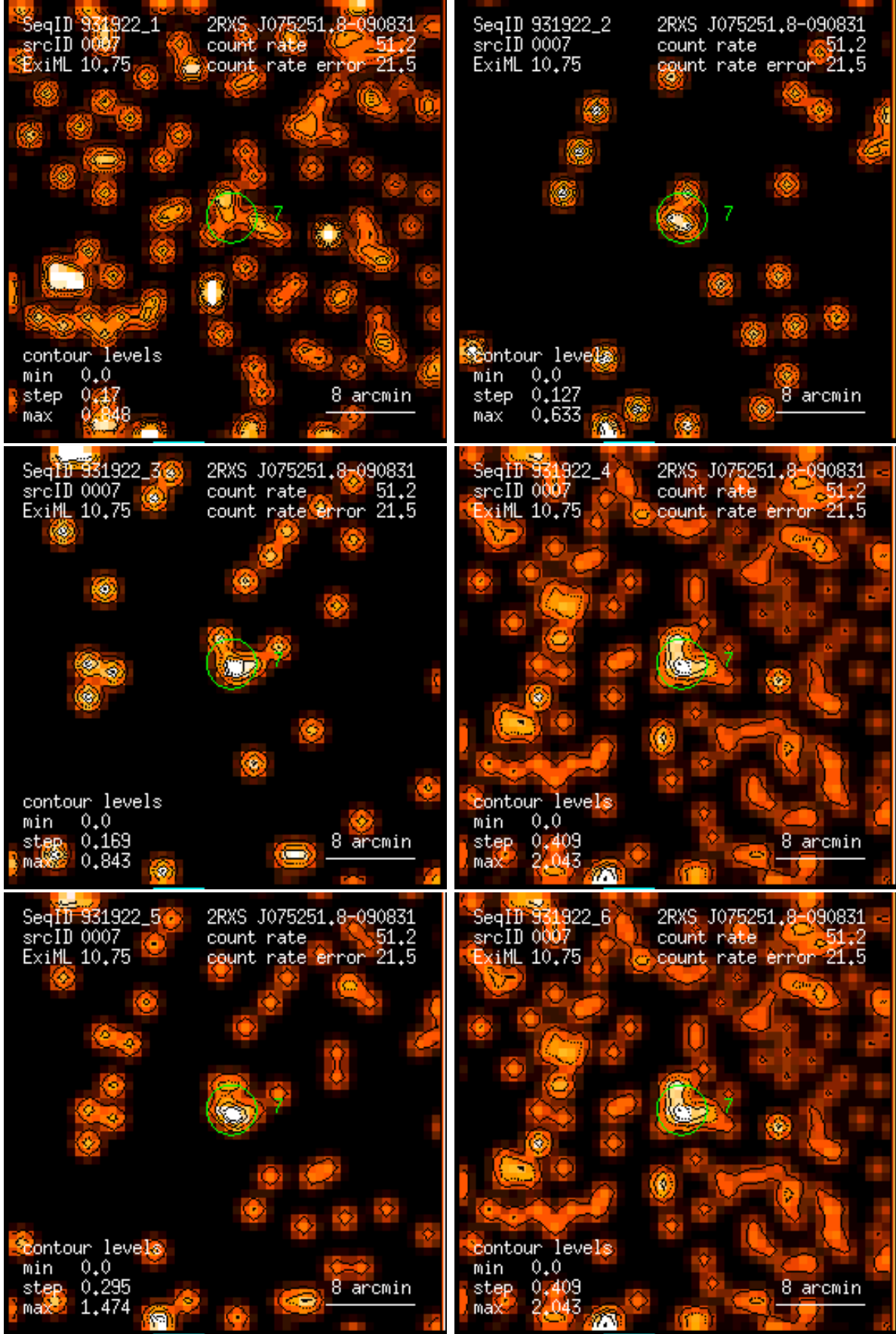
Figure 7: RASS 931922: detection 0007: band rate images, Gaussian filter: (1) PSPC channels 11 – 41, (2) 52 – 90, (3) 91 – 201, (4) 11 – 235, (5) 52 – 201, (6) 11 – 201. Broad band rates in counts/ks. Band rate contour levels in counts/ks/arcmin 2 .
