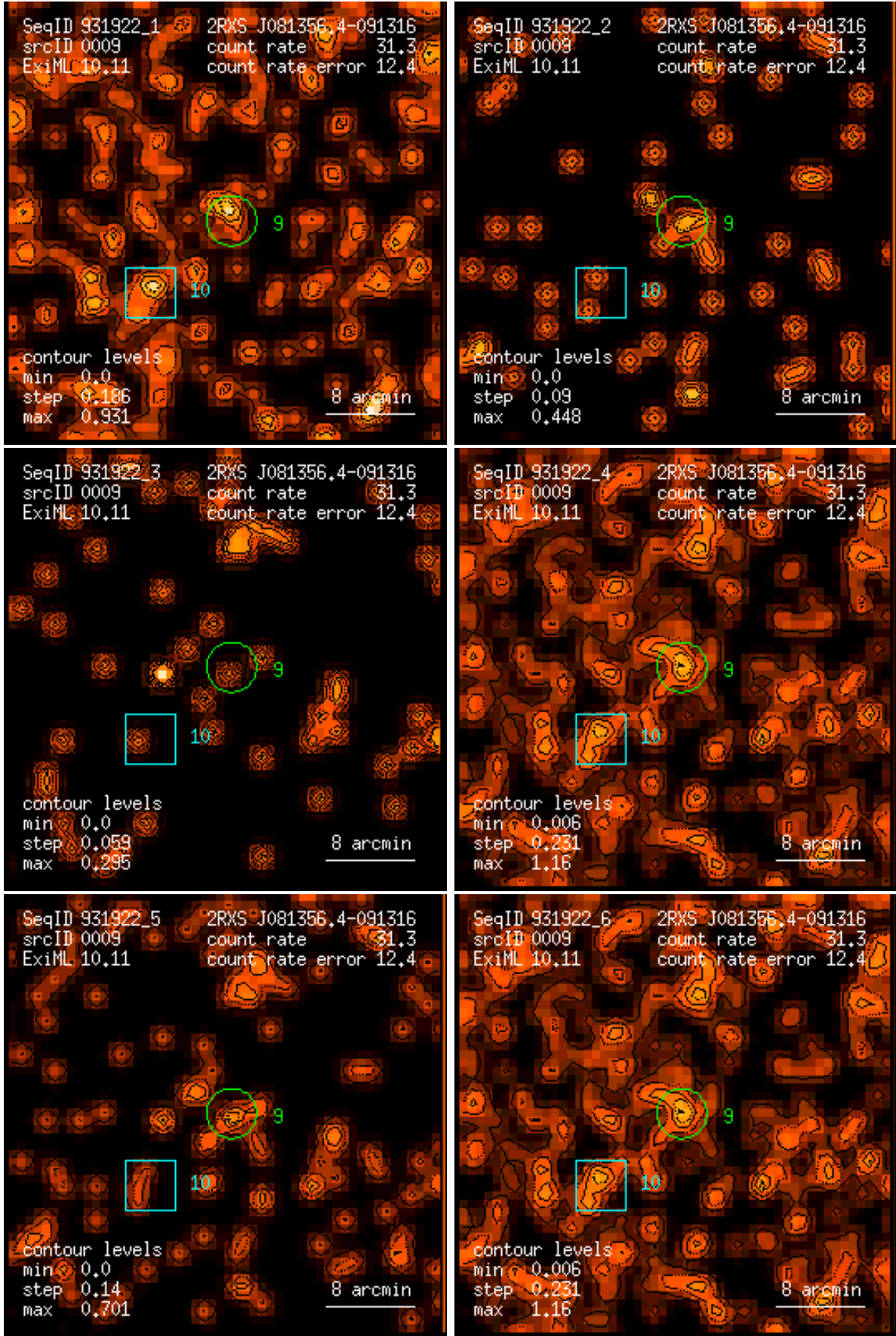
Figure 9: RASS 931922: detection 0009: band rate images, Gaussian filter: (1) PSPC channels 11 – 41, (2) 52 – 90, (3) 91 – 201, (4) 11 – 235, (5) 52 – 201, (6) 11 – 201. Broad band rates in counts/ks. Band rate contour levels in counts/ks/arcmin 2 .
