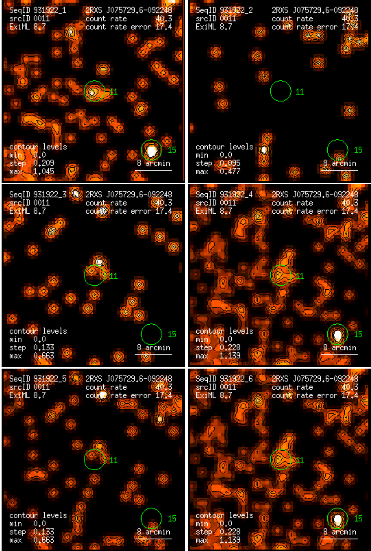
Figure 11: RASS 931922: detection 0011: band rate images, Gaussian filter: (1) PSPC channels 11 – 41, (2) 52 – 90, (3) 91 – 201, (4) 11 – 235, (5) 52 – 201, (6) 11 – 201. Broad band rates in counts/ks. Band rate contour levels in counts/ks/arcmin 2 .
