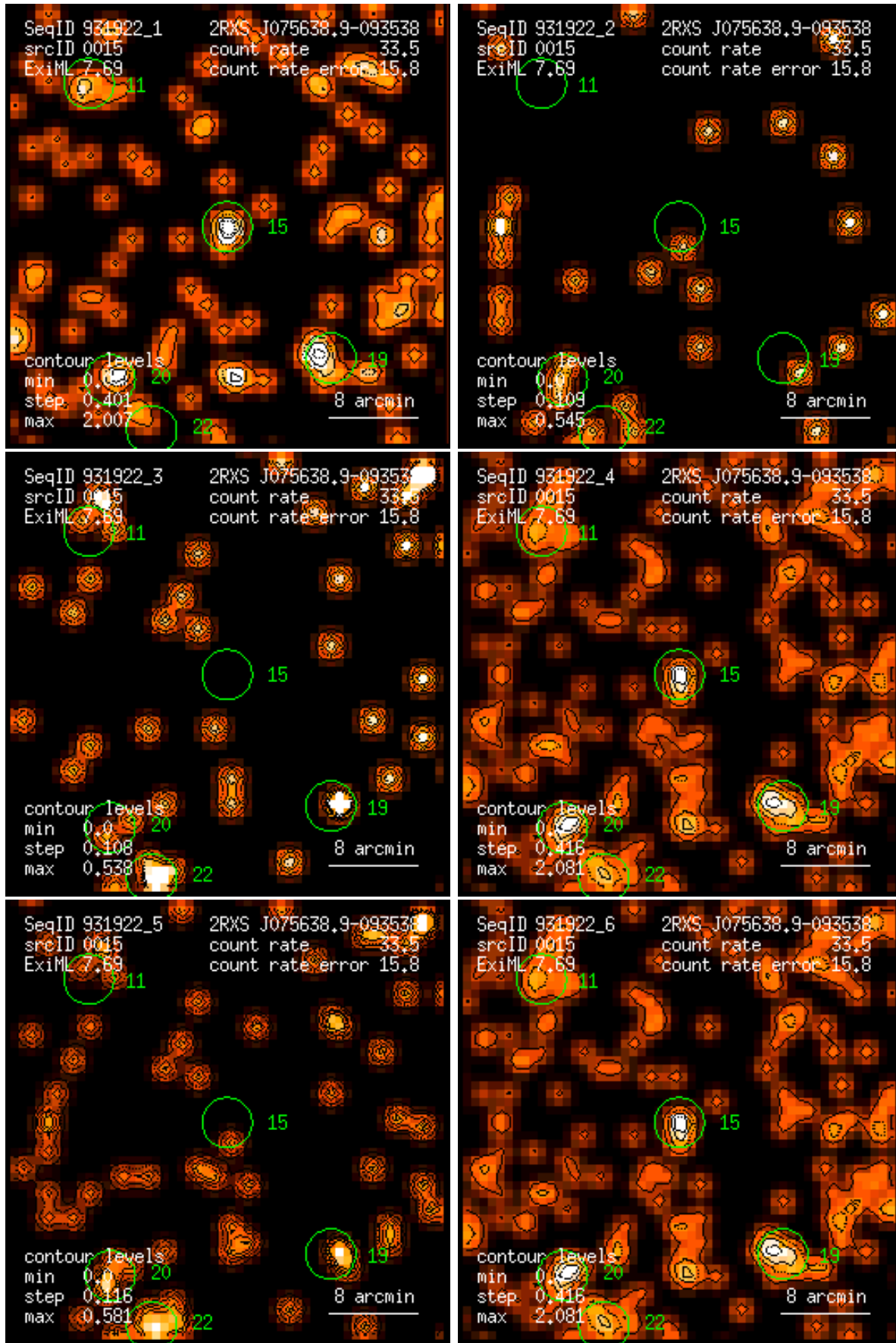
Figure 15: RASS 931922: detection 0015: band rate images, Gaussian filter: (1) PSPC channels 11 – 41, (2) 52 – 90, (3) 91 – 201, (4) 11 – 235, (5) 52 – 201, (6) 11 – 201. Broad band rates in counts/ks. Band rate contour levels in counts/ks/arcmin 2 .
