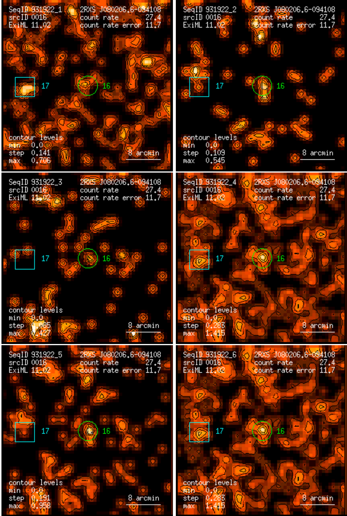
Figure 16: RASS 931922: detection 0016: band rate images, Gaussian filter: (1) PSPC channels 11 – 41, (2) 52 – 90, (3) 91 – 201, (4) 11 – 235, (5) 52 – 201, (6) 11 – 201. Broad band rates in counts/ks. Band rate contour levels in counts/ks/arcmin 2 .
