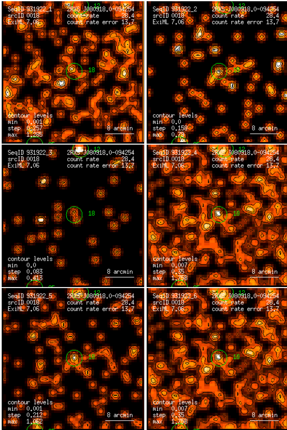
Figure 18: RASS 931922: detection 0018: band rate images, Gaussian filter: (1) PSPC channels 11 – 41, (2) 52 – 90, (3) 91 – 201, (4) 11 – 235, (5) 52 – 201, (6) 11 – 201. Broad band rates in counts/ks. Band rate contour levels in counts/ks/arcmin 2 .
