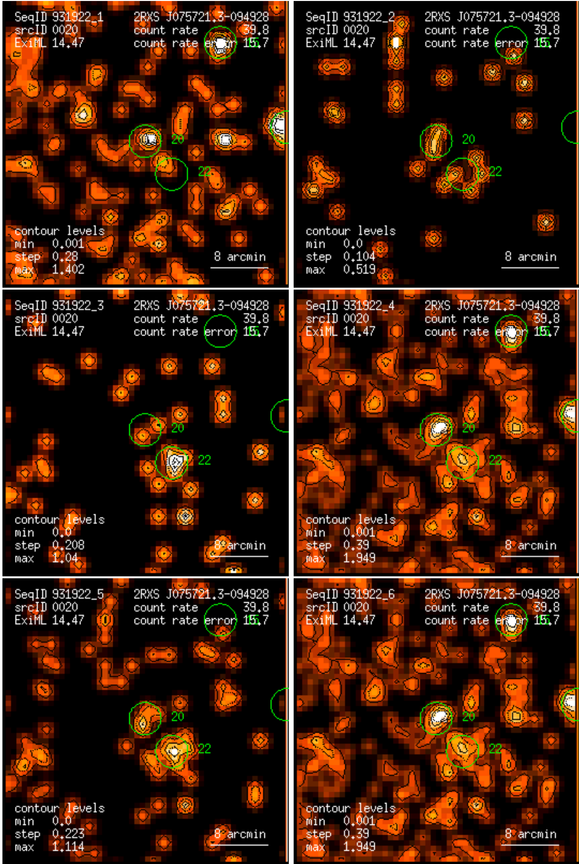
Figure 20: RASS 931922: detection 0020: band rate images, Gaussian filter: (1) PSPC channels 11 – 41, (2) 52 – 90, (3) 91 – 201, (4) 11 – 235, (5) 52 – 201, (6) 11 – 201. Broad band rates in counts/ks. Band rate contour levels in counts/ks/arcmin 2 .
