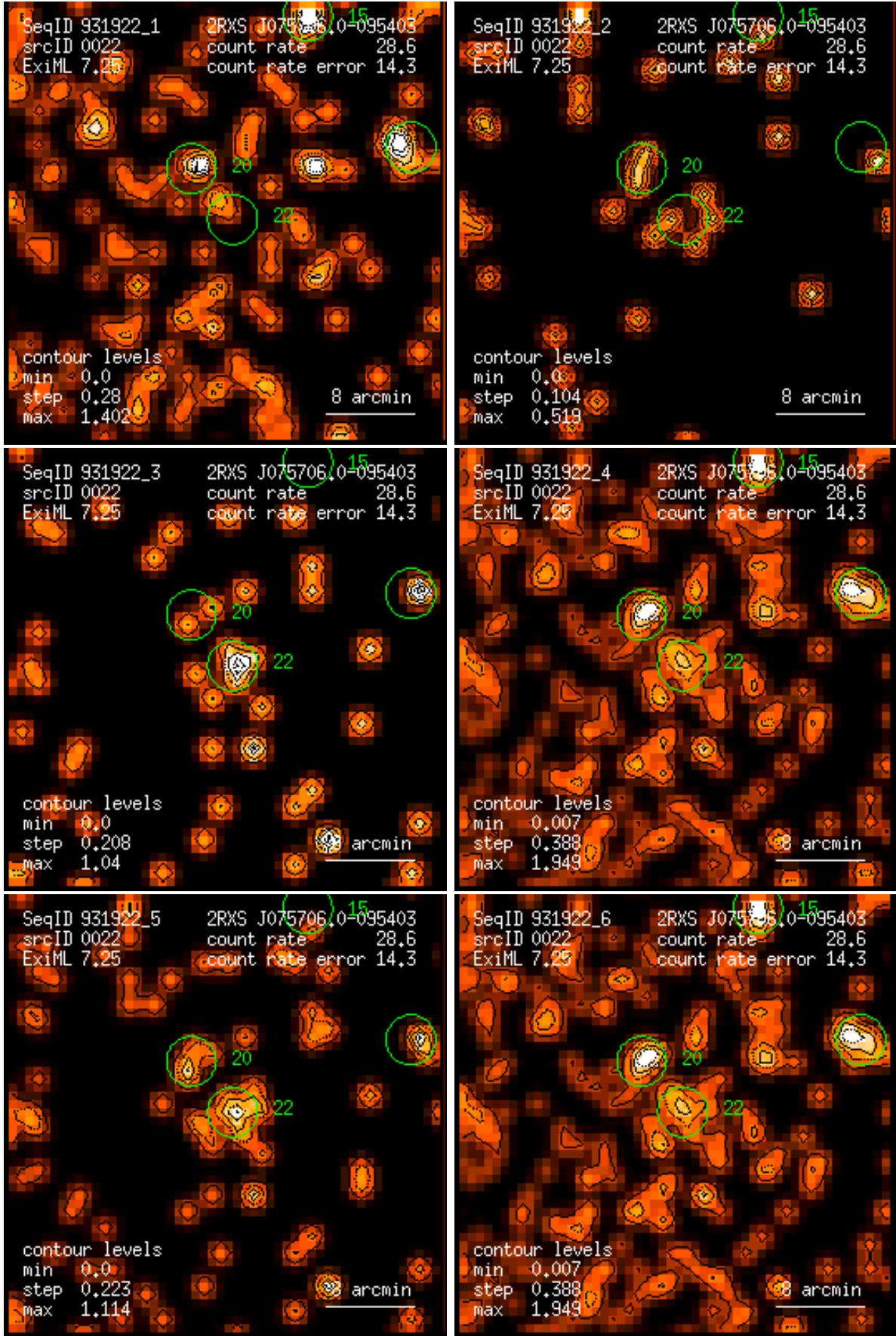
Figure 22: RASS 931922: detection 0022: band rate images, Gaussian filter: (1) PSPC channels 11 – 41, (2) 52 – 90, (3) 91 – 201, (4) 11 – 235, (5) 52 – 201, (6) 11 – 201. Broad band rates in counts/ks. Band rate contour levels in counts/ks/arcmin 2 .
