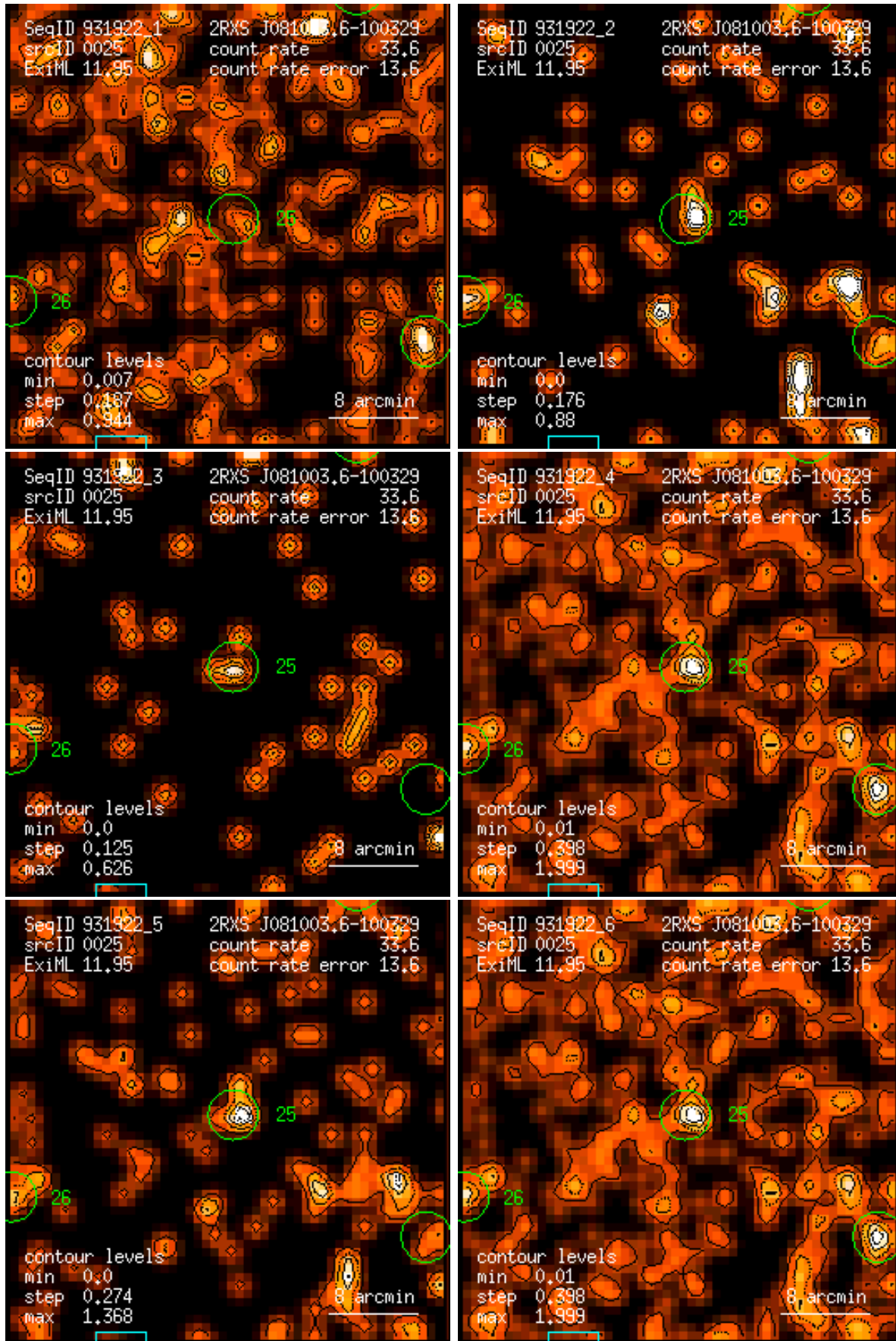
Figure 25: RASS 931922: detection 0025: band rate images, Gaussian filter: (1) PSPC channels 11 – 41, (2) 52 – 90, (3) 91 – 201, (4) 11 – 235, (5) 52 – 201, (6) 11 – 201. Broad band rates in counts/ks. Band rate contour levels in counts/ks/arcmin 2 .
