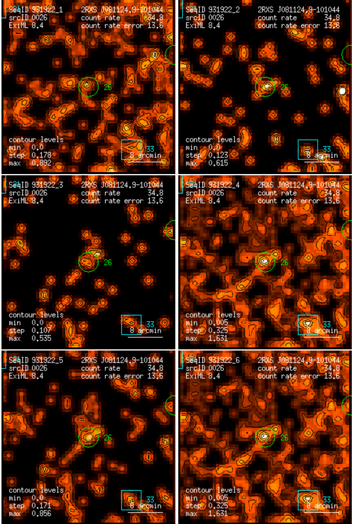
Figure 26: RASS 931922: detection 0026: band rate images, Gaussian filter: (1) PSPC channels 11 – 41, (2) 52 – 90, (3) 91 – 201, (4) 11 – 235, (5) 52 – 201, (6) 11 – 201. Broad band rates in counts/ks. Band rate contour levels in counts/ks/arcmin 2 .
