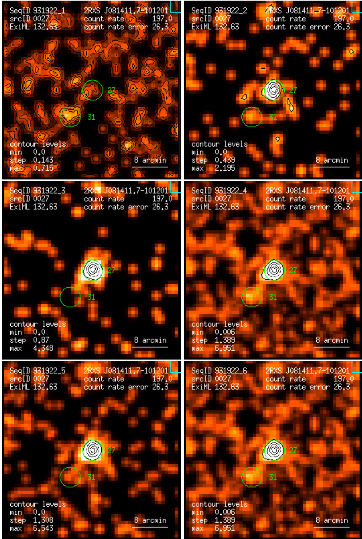
Figure 27: RASS 931922: detection 0027: band rate images, Gaussian filter: (1) PSPC channels 11 – 41, (2) 52 – 90, (3) 91 – 201, (4) 11 – 235, (5) 52 – 201, (6) 11 – 201. Broad band rates in counts/ks. Band rate contour levels in counts/ks/arcmin 2 .
