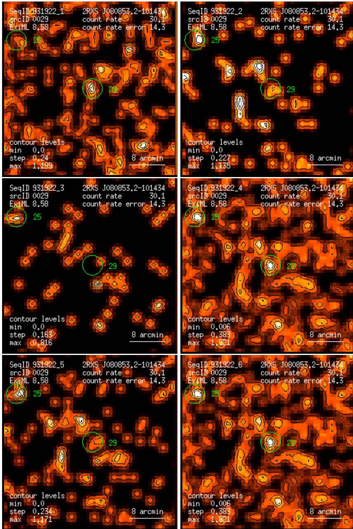
Figure 29: RASS 931922: detection 0029: band rate images, Gaussian filter: (1) PSPC channels 11 – 41, (2) 52 – 90, (3) 91 – 201, (4) 11 – 235, (5) 52 – 201, (6) 11 – 201. Broad band rates in counts/ks. Band rate contour levels in counts/ks/arcmin 2 .
