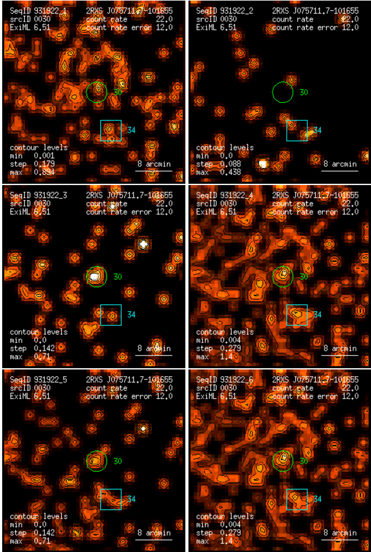
Figure 30: RASS 931922: detection 0030: band rate images, Gaussian filter: (1) PSPC channels 11 – 41, (2) 52 – 90, (3) 91 – 201, (4) 11 – 235, (5) 52 – 201, (6) 11 – 201. Broad band rates in counts/ks. Band rate contour levels in counts/ks/arcmin 2 .
