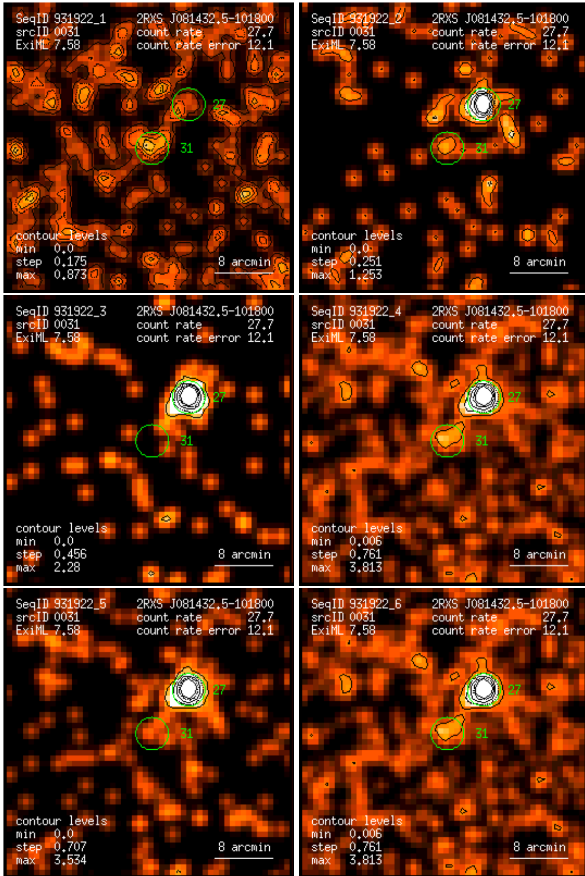
Figure 31: RASS 931922: detection 0031: band rate images, Gaussian filter: (1) PSPC channels 11 – 41, (2) 52 – 90, (3) 91 – 201, (4) 11 – 235, (5) 52 – 201, (6) 11 – 201. Broad band rates in counts/ks. Band rate contour levels in counts/ks/arcmin 2 .
