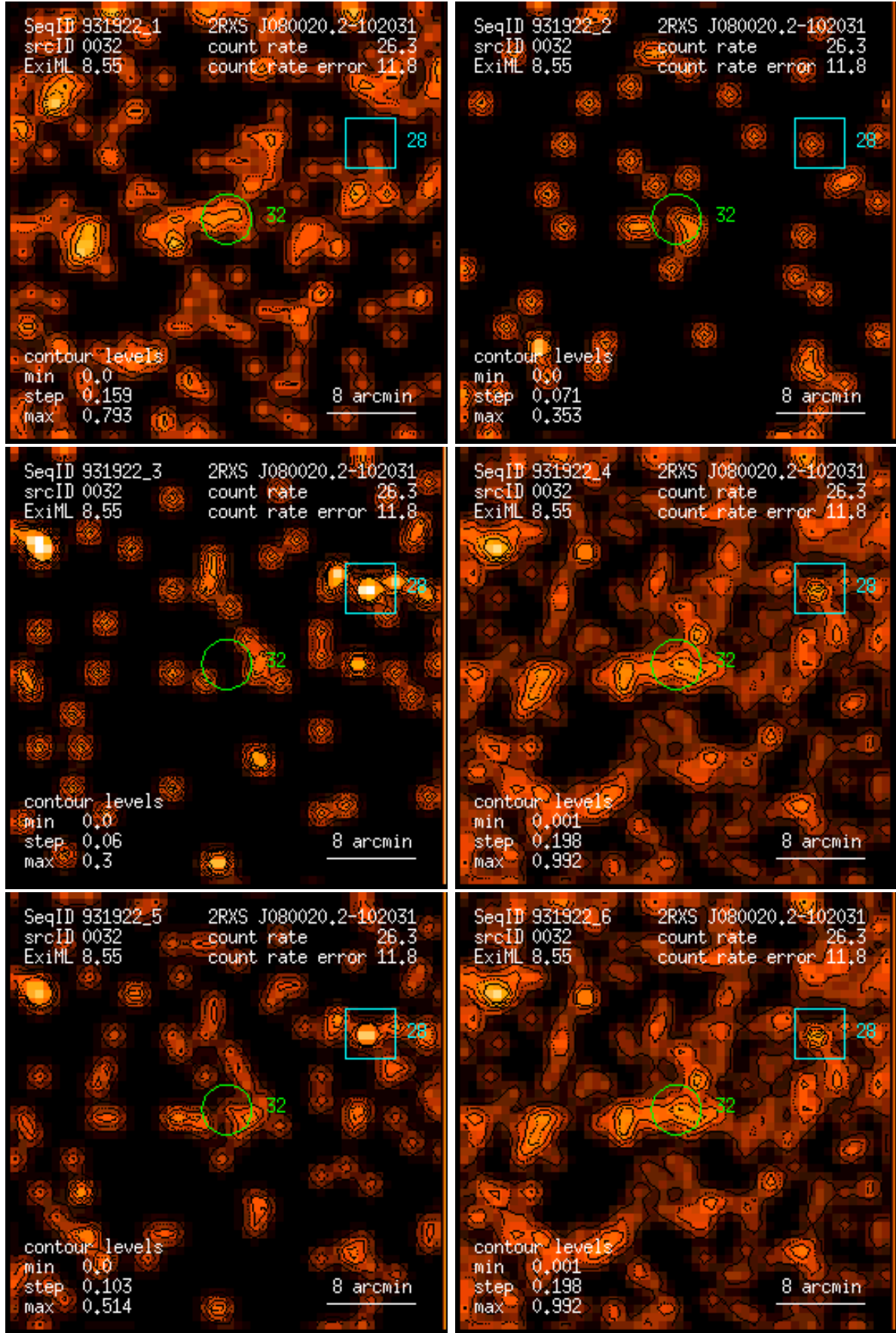
Figure 32: RASS 931922: detection 0032: band rate images, Gaussian filter: (1) PSPC channels 11 – 41, (2) 52 – 90, (3) 91 – 201, (4) 11 – 235, (5) 52 – 201, (6) 11 – 201. Broad band rates in counts/ks. Band rate contour levels in counts/ks/arcmin 2 .
