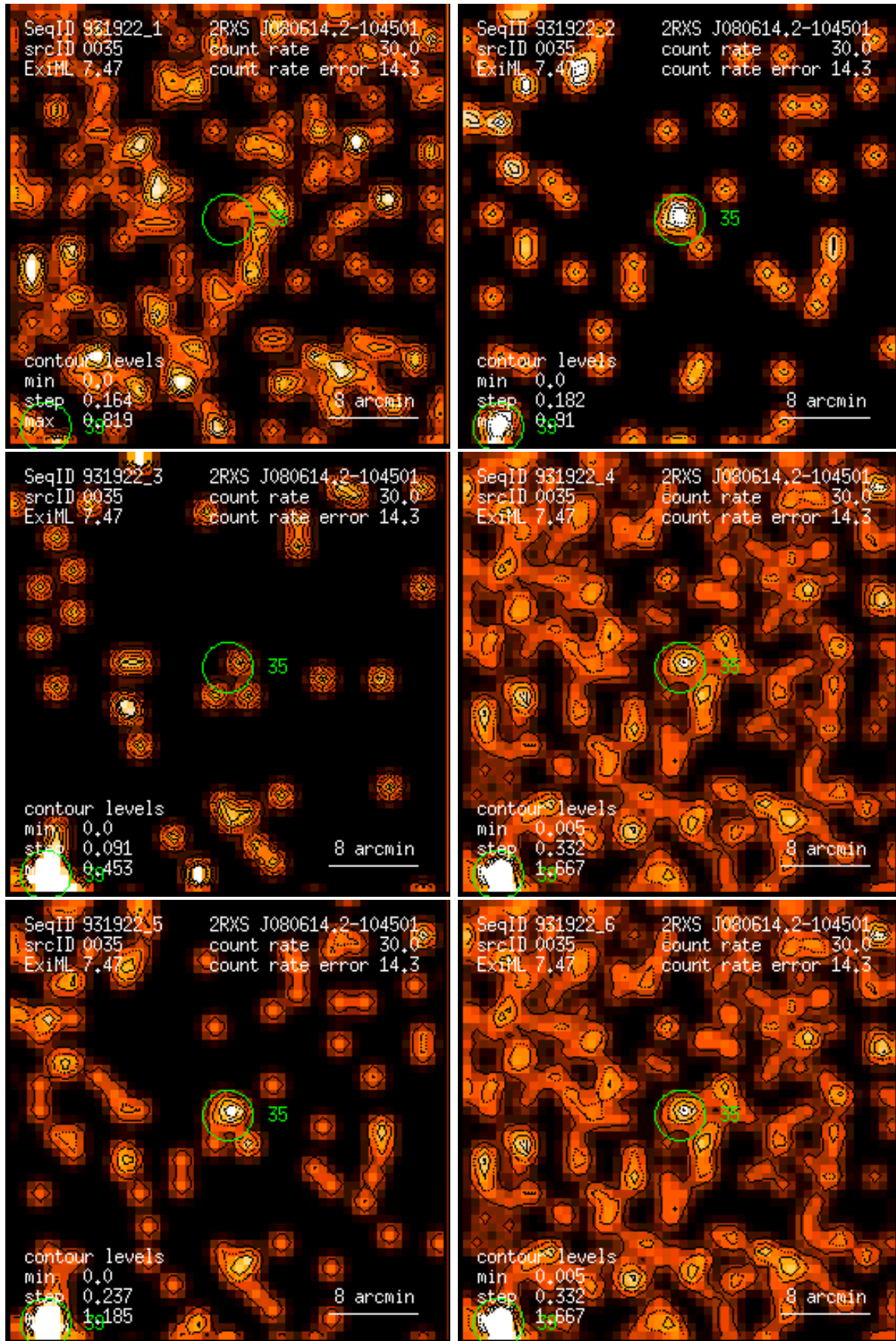
Figure 35: RASS 931922: detection 0035: band rate images, Gaussian filter: (1) PSPC channels 11 – 41, (2) 52 – 90, (3) 91 – 201, (4) 11 – 235, (5) 52 – 201, (6) 11 – 201. Broad band rates in counts/ks. Band rate contour levels in counts/ks/arcmin 2 .
