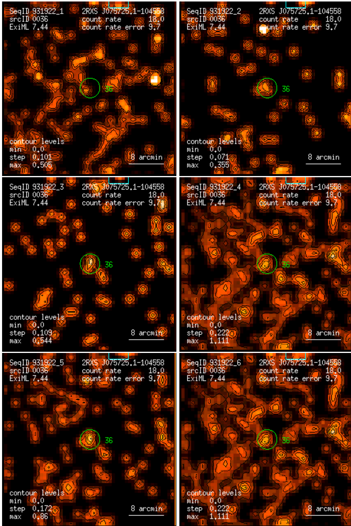
Figure 36: RASS 931922: detection 0036: band rate images, Gaussian filter: (1) PSPC channels 11 – 41, (2) 52 – 90, (3) 91 – 201, (4) 11 – 235, (5) 52 – 201, (6) 11 – 201. Broad band rates in counts/ks. Band rate contour levels in counts/ks/arcmin 2 .
