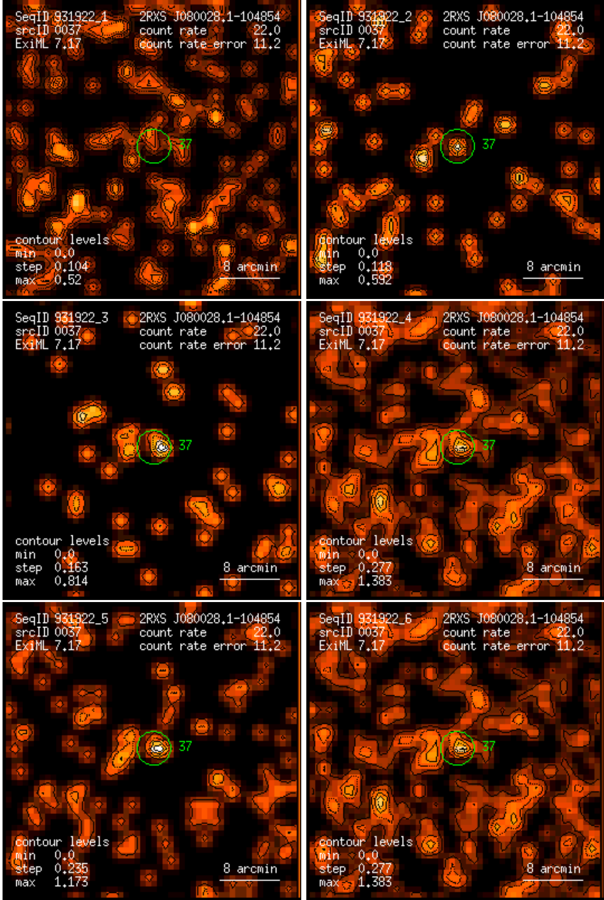
Figure 37: RASS 931922: detection 0037: band rate images, Gaussian filter: (1) PSPC channels 11 – 41, (2) 52 – 90, (3) 91 – 201, (4) 11 – 235, (5) 52 – 201, (6) 11 – 201. Broad band rates in counts/ks. Band rate contour levels in counts/ks/arcmin 2 .
