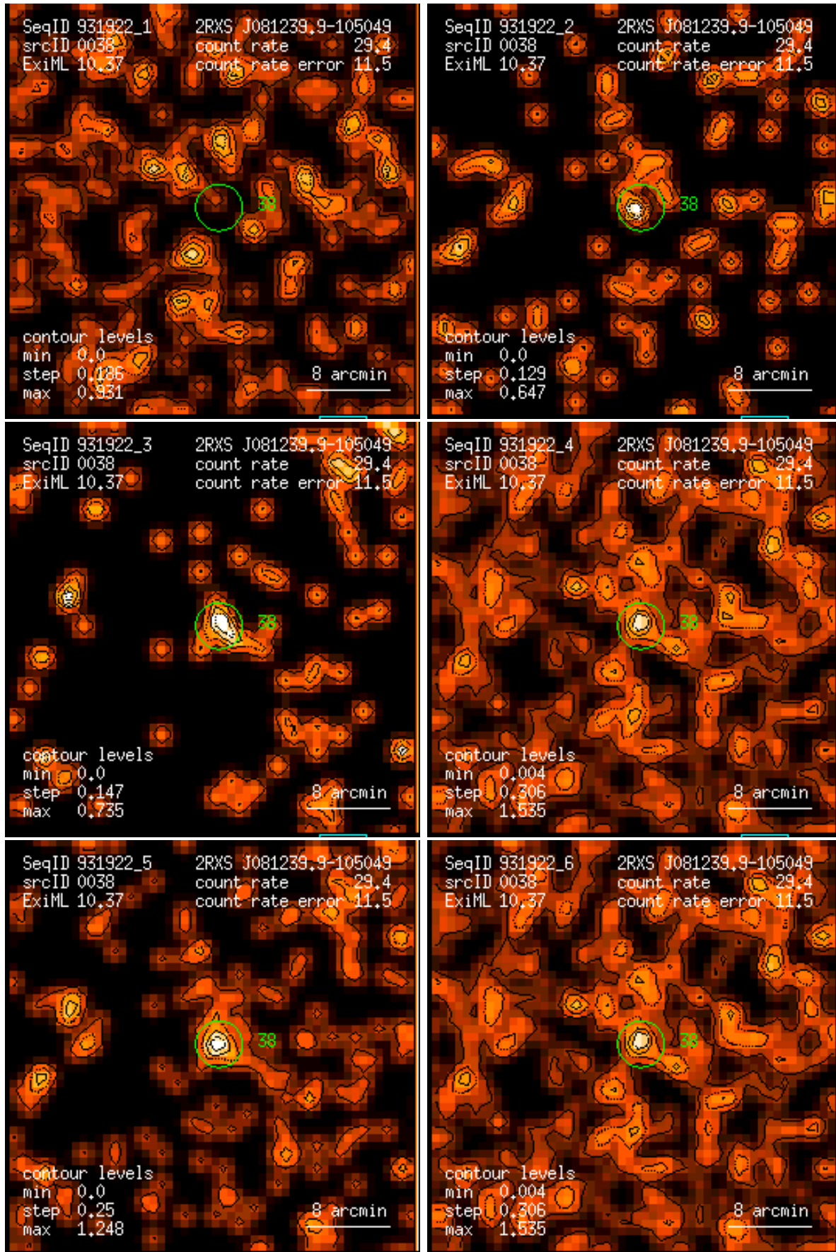
Figure 38: RASS 931922: detection 0038: band rate images, Gaussian filter: (1) PSPC channels 11 – 41, (2) 52 – 90, (3) 91 – 201, (4) 11 – 235, (5) 52 – 201, (6) 11 – 201. Broad band rates in counts/ks. Band rate contour levels in counts/ks/arcmin 2 .
