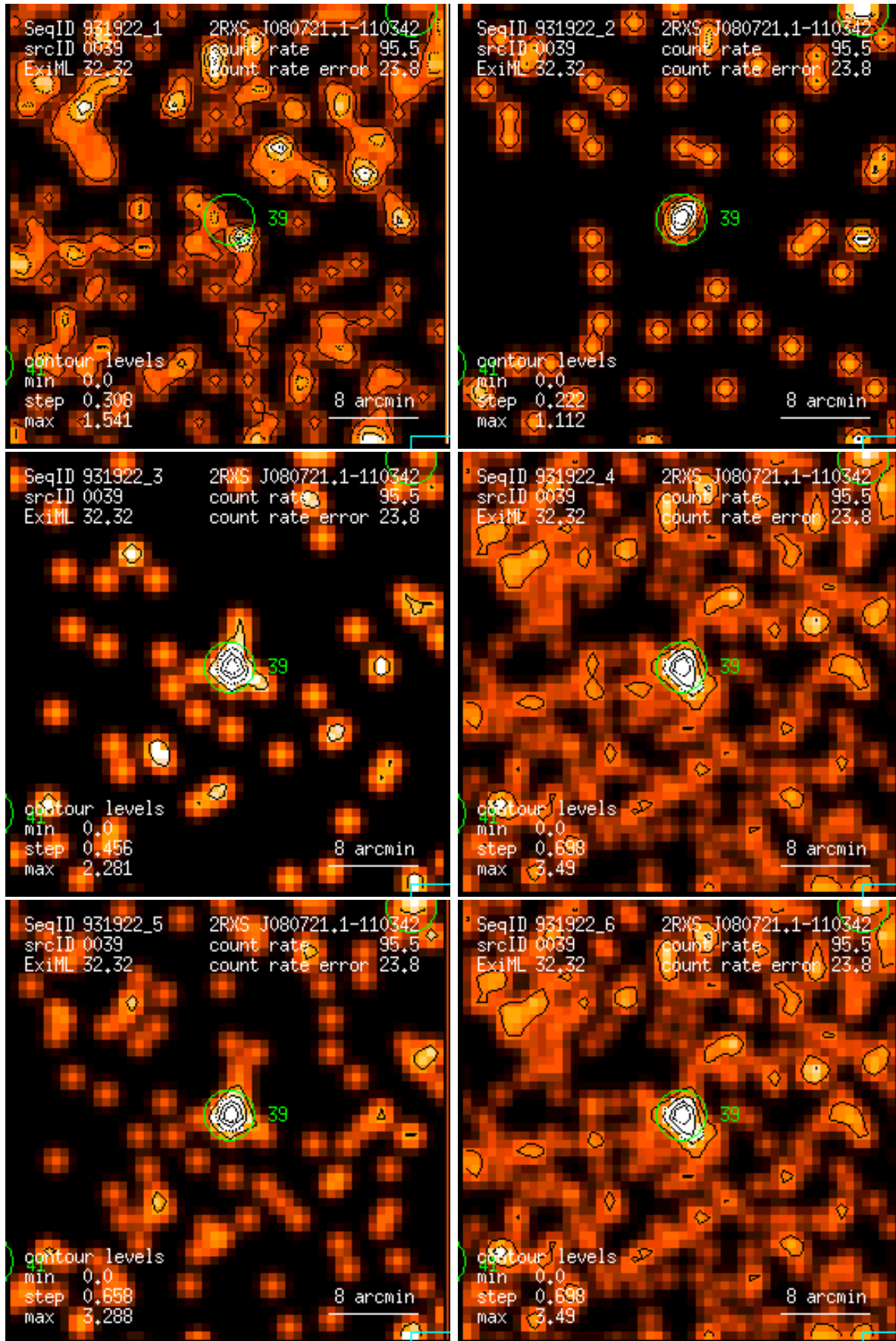
Figure 39: RASS 931922: detection 0039: band rate images, Gaussian filter: (1) PSPC channels 11 – 41, (2) 52 – 90, (3) 91 – 201, (4) 11 – 235, (5) 52 – 201, (6) 11 – 201. Broad band rates in counts/ks. Band rate contour levels in counts/ks/arcmin 2 .
