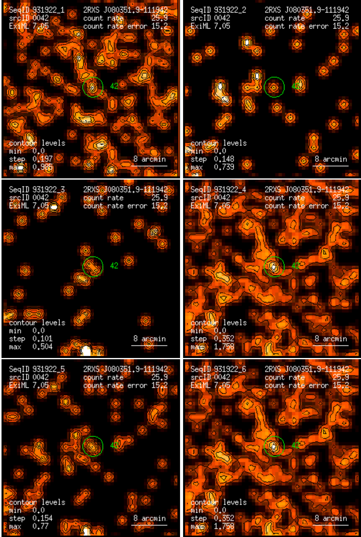
Figure 42: RASS 931922: detection 0042: band rate images, Gaussian filter: (1) PSPC channels 11 – 41, (2) 52 – 90, (3) 91 – 201, (4) 11 – 235, (5) 52 – 201, (6) 11 – 201. Broad band rates in counts/ks. Band rate contour levels in counts/ks/arcmin 2 .
