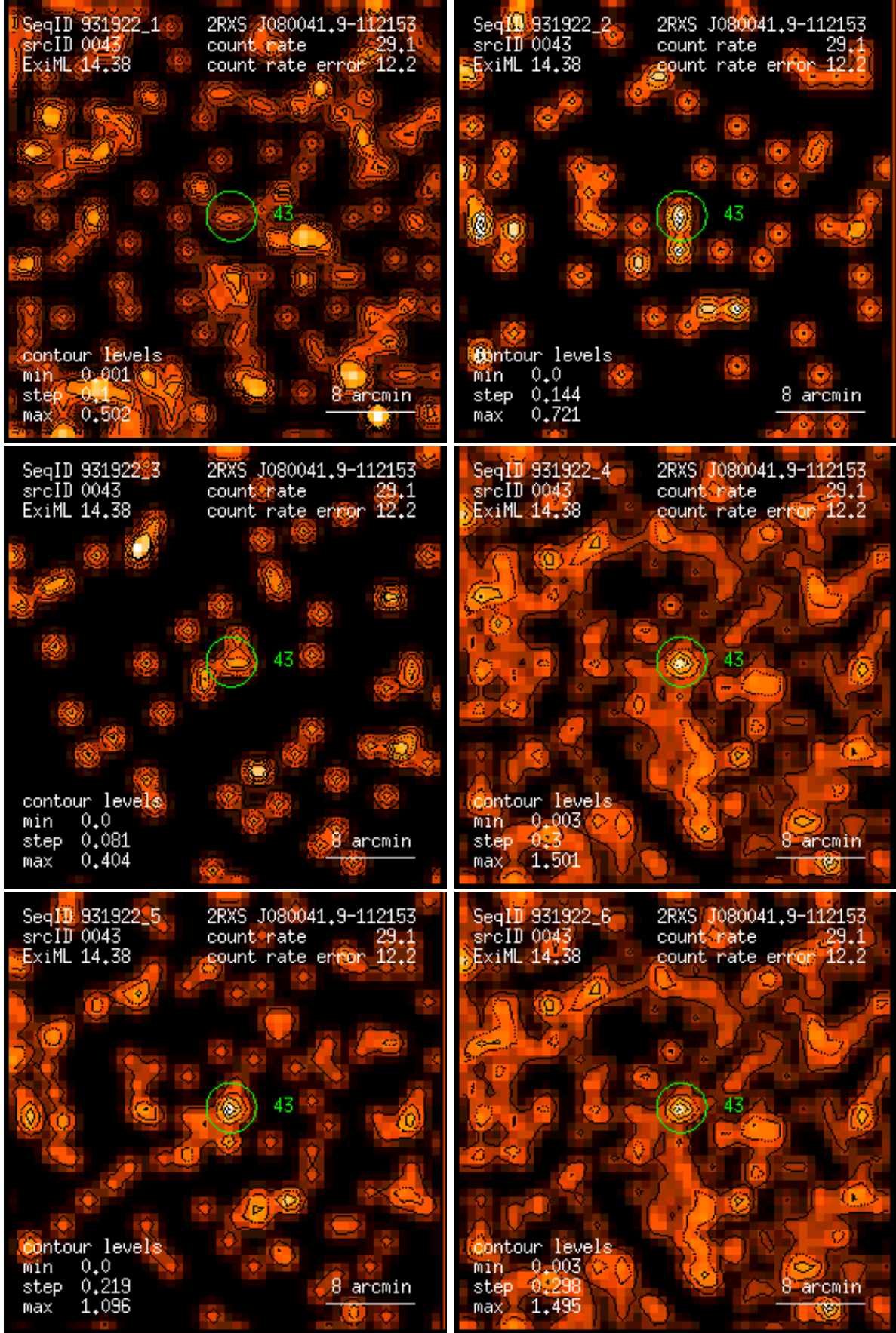
Figure 43: RASS 931922: detection 0043: band rate images, Gaussian filter: (1) PSPC channels 11 – 41, (2) 52 – 90, (3) 91 – 201, (4) 11 – 235, (5) 52 – 201, (6) 11 – 201. Broad band rates in counts/ks. Band rate contour levels in counts/ks/arcmin 2 .
