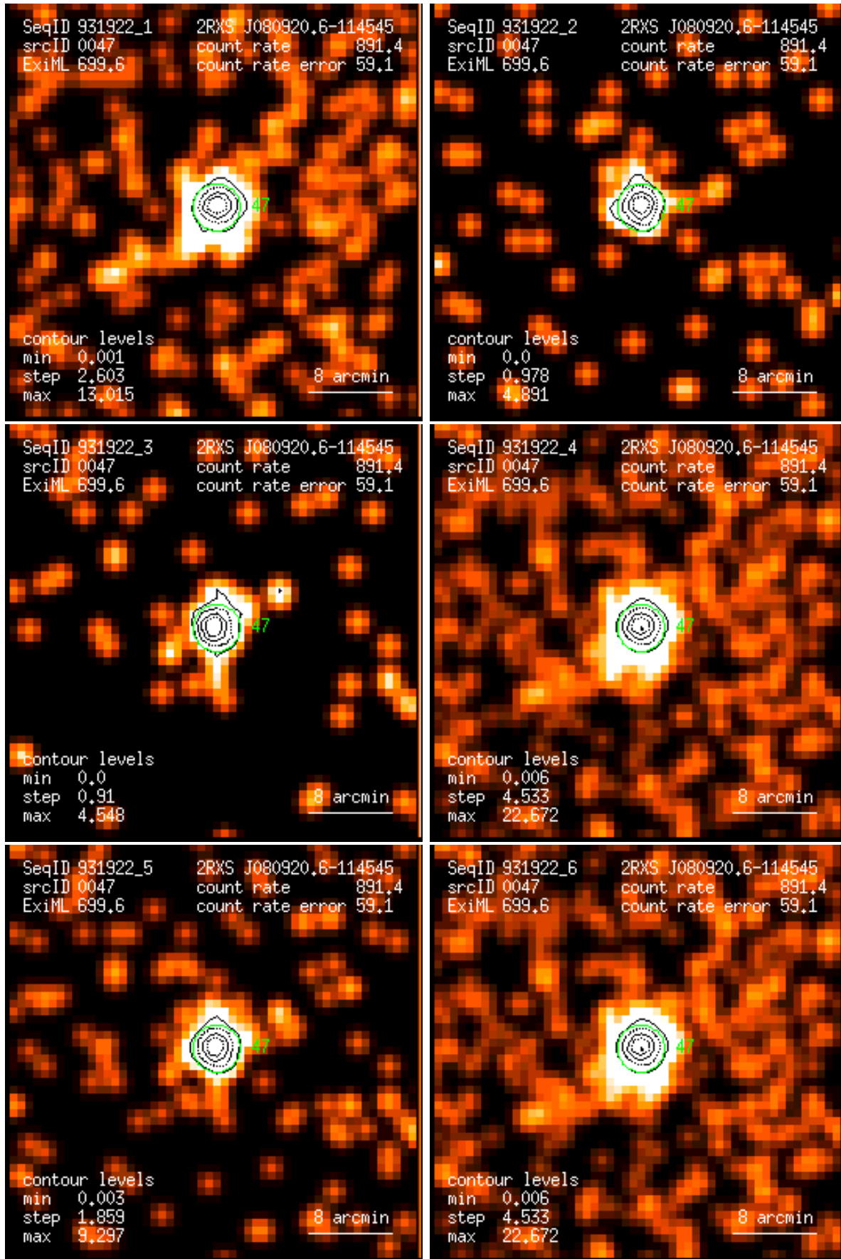
Figure 47: RASS 931922: detection 0047: band rate images, Gaussian filter: (1) PSPC channels 11 – 41, (2) 52 – 90, (3) 91 – 201, (4) 11 – 235, (5) 52 – 201, (6) 11 – 201. Broad band rates in counts/ks. Band rate contour levels in counts/ks/arcmin 2 .
