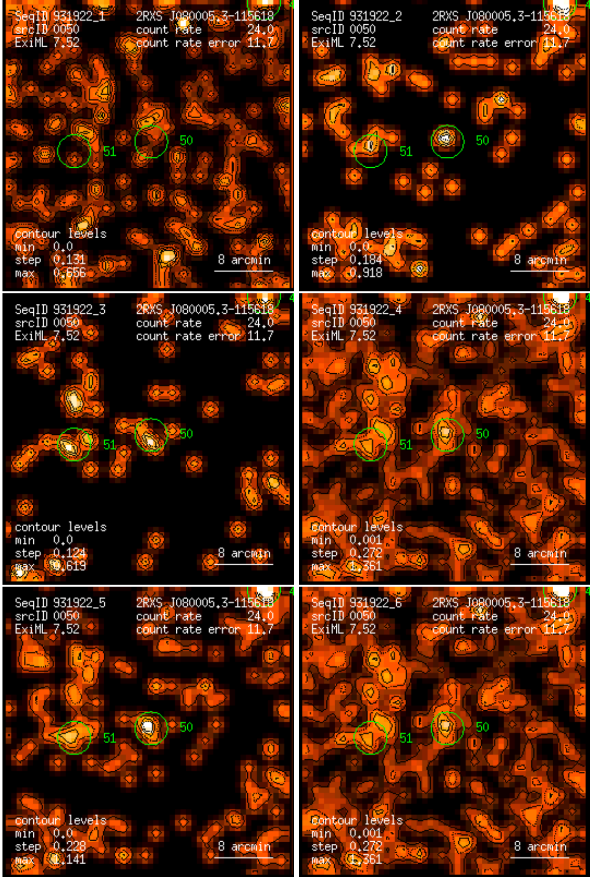
Figure 50: RASS 931922: detection 0050: band rate images, Gaussian filter: (1) PSPC channels 11 – 41, (2) 52 – 90, (3) 91 – 201, (4) 11 – 235, (5) 52 – 201, (6) 11 – 201. Broad band rates in counts/ks. Band rate contour levels in counts/ks/arcmin 2 .
