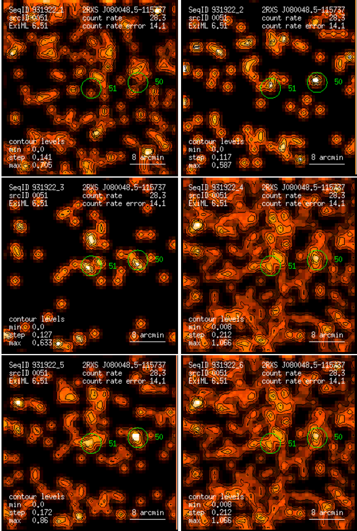
Figure 51: RASS 931922: detection 0051: band rate images, Gaussian filter: (1) PSPC channels 11 – 41, (2) 52 – 90, (3) 91 – 201, (4) 11 – 235, (5) 52 – 201, (6) 11 – 201. Broad band rates in counts/ks. Band rate contour levels in counts/ks/arcmin 2 .
