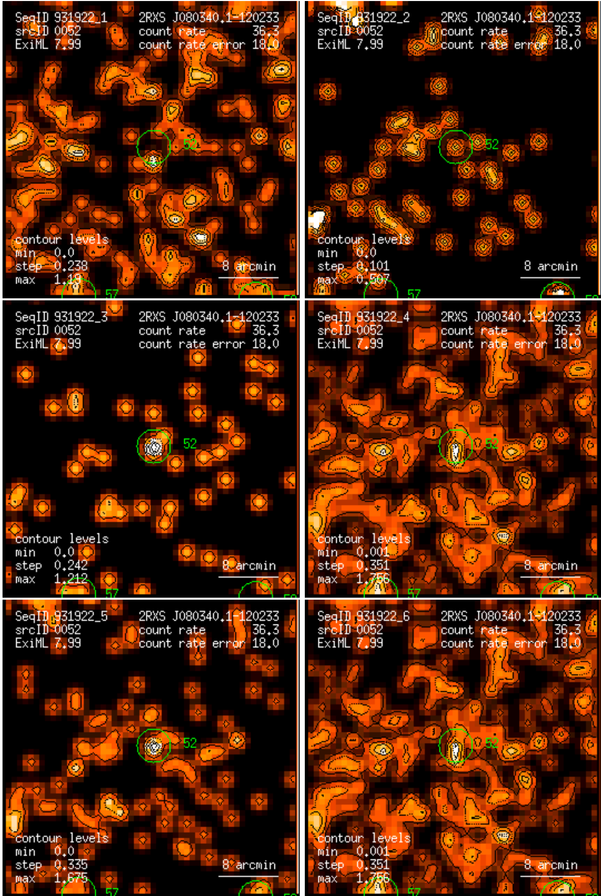
Figure 52: RASS 931922: detection 0052: band rate images, Gaussian filter: (1) PSPC channels 11 – 41, (2) 52 – 90, (3) 91 – 201, (4) 11 – 235, (5) 52 – 201, (6) 11 – 201. Broad band rates in counts/ks. Band rate contour levels in counts/ks/arcmin 2 .
