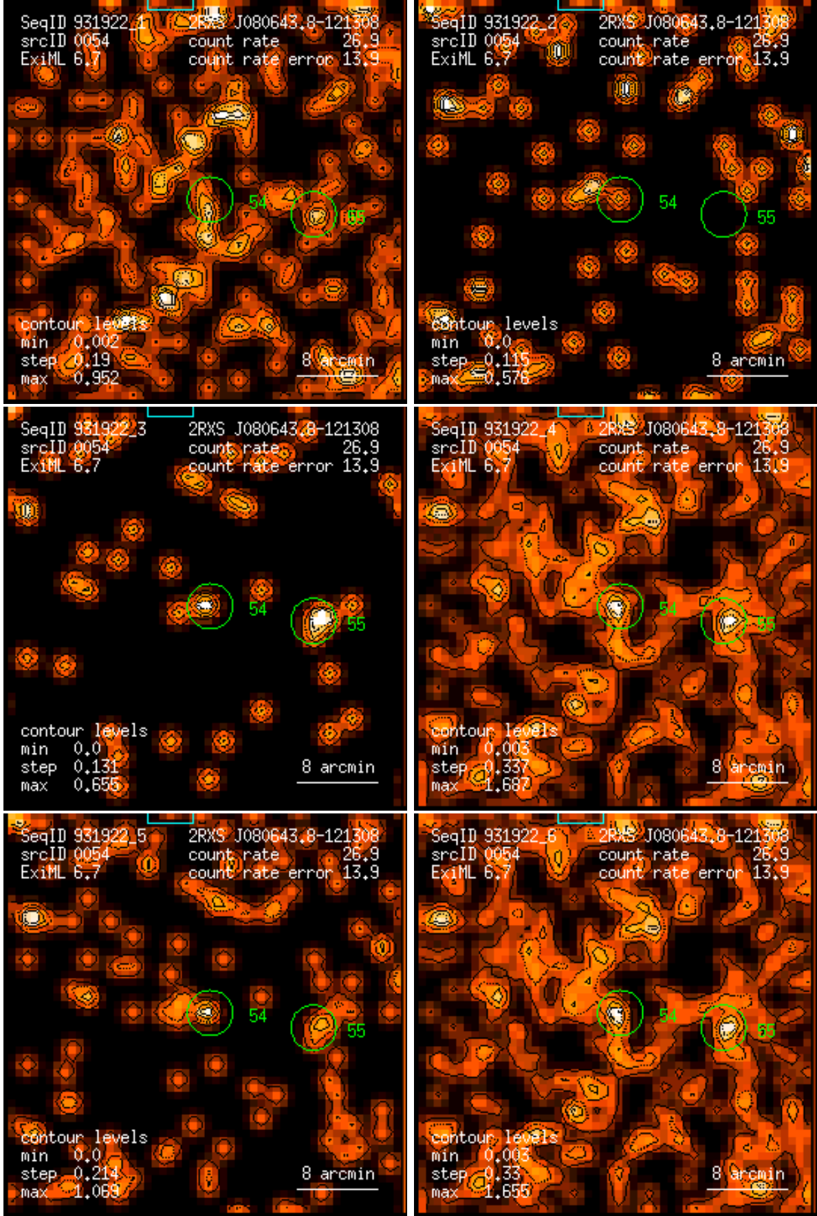
Figure 54: RASS 931922: detection 0054: band rate images, Gaussian filter: (1) PSPC channels 11 – 41, (2) 52 – 90, (3) 91 – 201, (4) 11 – 235, (5) 52 – 201, (6) 11 – 201. Broad band rates in counts/ks. Band rate contour levels in counts/ks/arcmin 2 .
