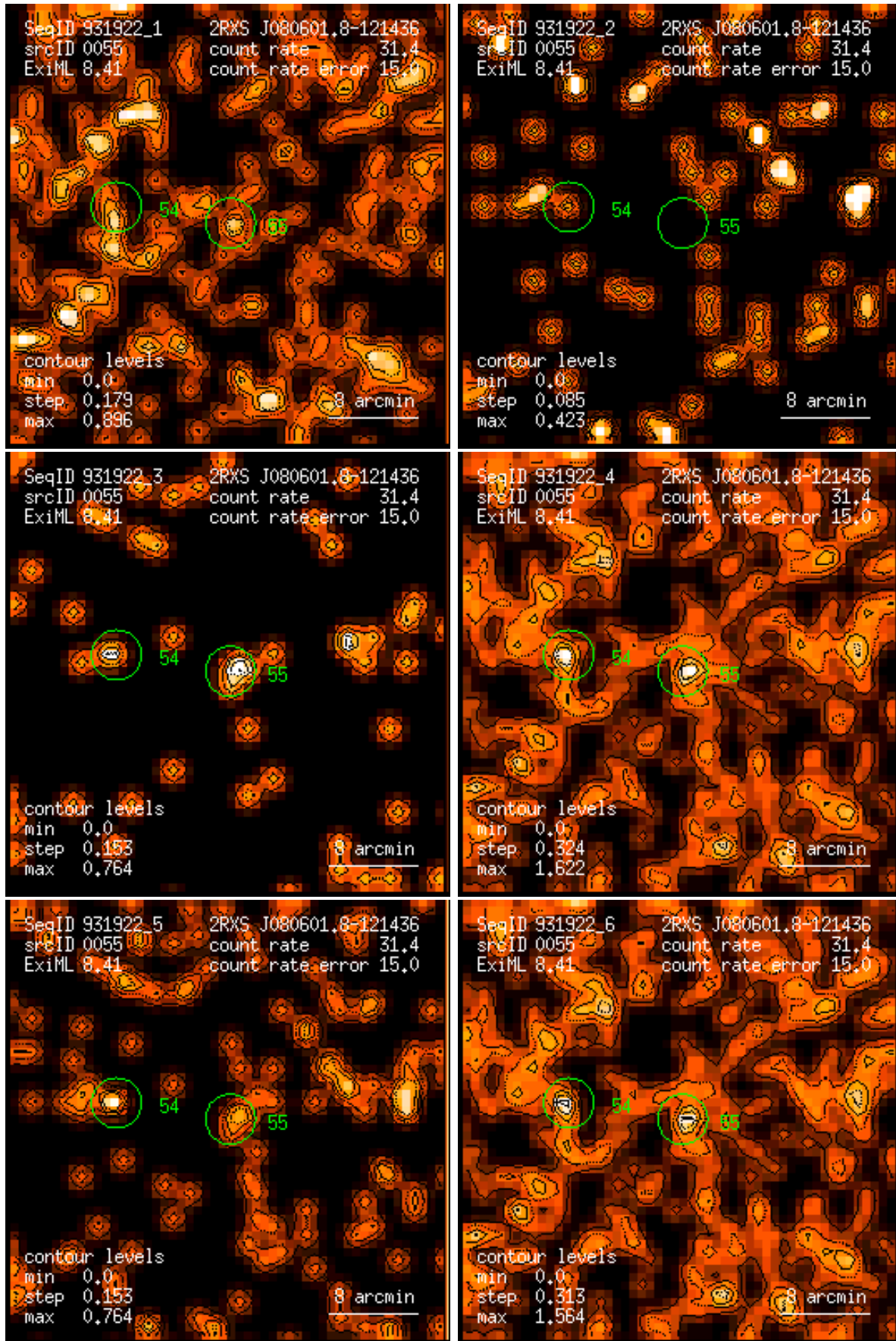
Figure 55: RASS 931922: detection 0055: band rate images, Gaussian filter: (1) PSPC channels 11 – 41, (2) 52 – 90, (3) 91 – 201, (4) 11 – 235, (5) 52 – 201, (6) 11 – 201. Broad band rates in counts/ks. Band rate contour levels in counts/ks/arcmin 2 .
