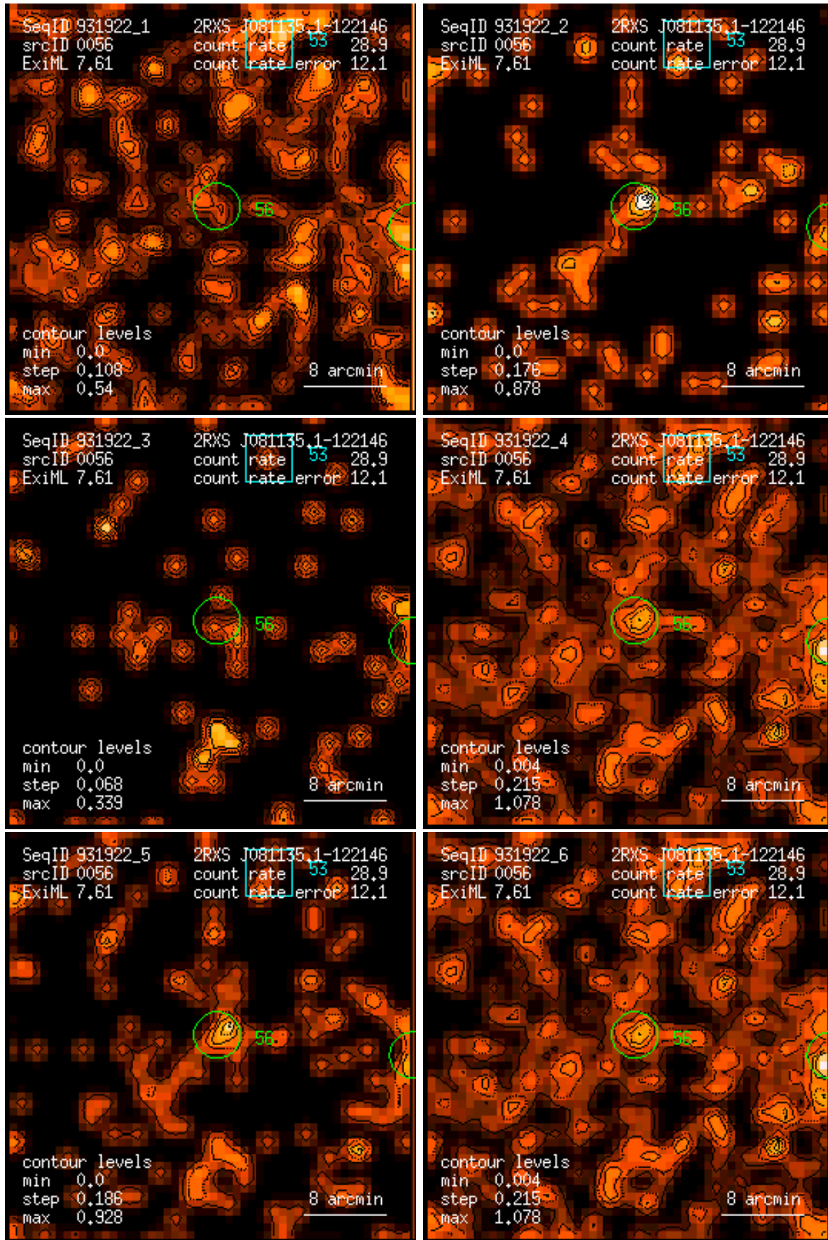
Figure 56: RASS 931922: detection 0056: band rate images, Gaussian filter: (1) PSPC channels 11 – 41, (2) 52 – 90, (3) 91 – 201, (4) 11 – 235, (5) 52 – 201, (6) 11 – 201. Broad band rates in counts/ks. Band rate contour levels in counts/ks/arcmin 2 .
