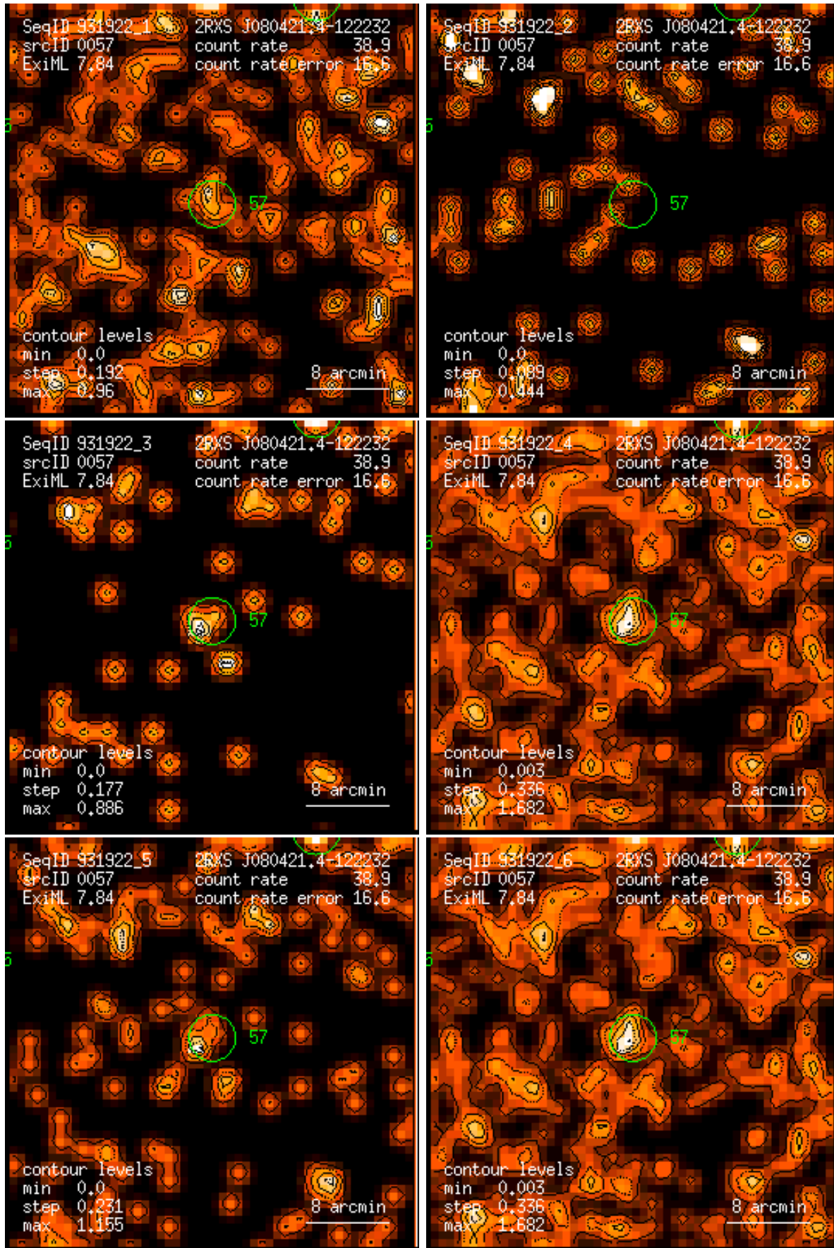
Figure 57: RASS 931922: detection 0057: band rate images, Gaussian filter: (1) PSPC channels 11 – 41, (2) 52 – 90, (3) 91 – 201, (4) 11 – 235, (5) 52 – 201, (6) 11 – 201. Broad band rates in counts/ks. Band rate contour levels in counts/ks/arcmin 2 .
