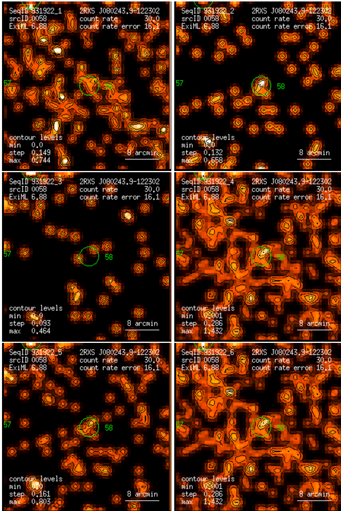
Figure 58: RASS 931922: detection 0058: band rate images, Gaussian filter: (1) PSPC channels 11 – 41, (2) 52 – 90, (3) 91 – 201, (4) 11 – 235, (5) 52 – 201, (6) 11 – 201. Broad band rates in counts/ks. Band rate contour levels in counts/ks/arcmin 2 .
