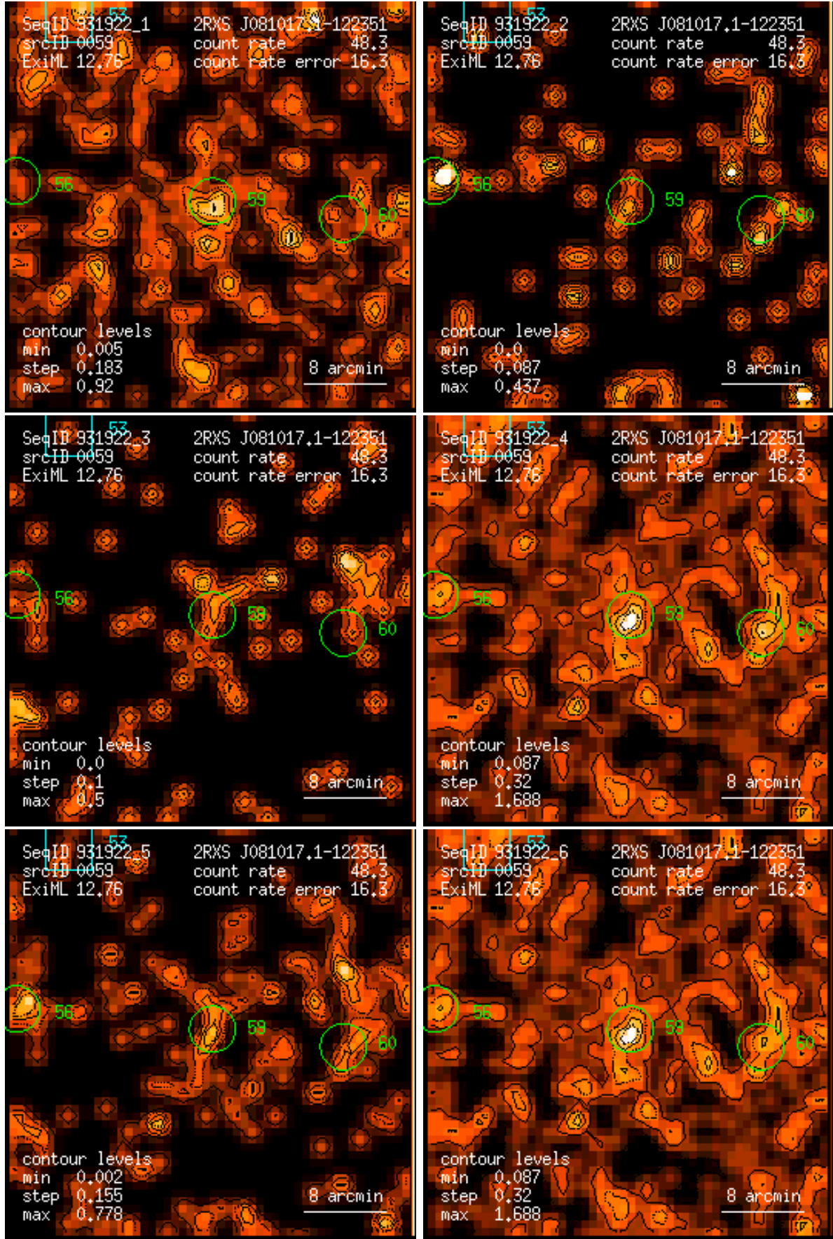
Figure 59: RASS 931922: detection 0059: band rate images, Gaussian filter: (1) PSPC channels 11 – 41, (2) 52 – 90, (3) 91 – 201, (4) 11 – 235, (5) 52 – 201, (6) 11 – 201. Broad band rates in counts/ks. Band rate contour levels in counts/ks/arcmin 2 .
