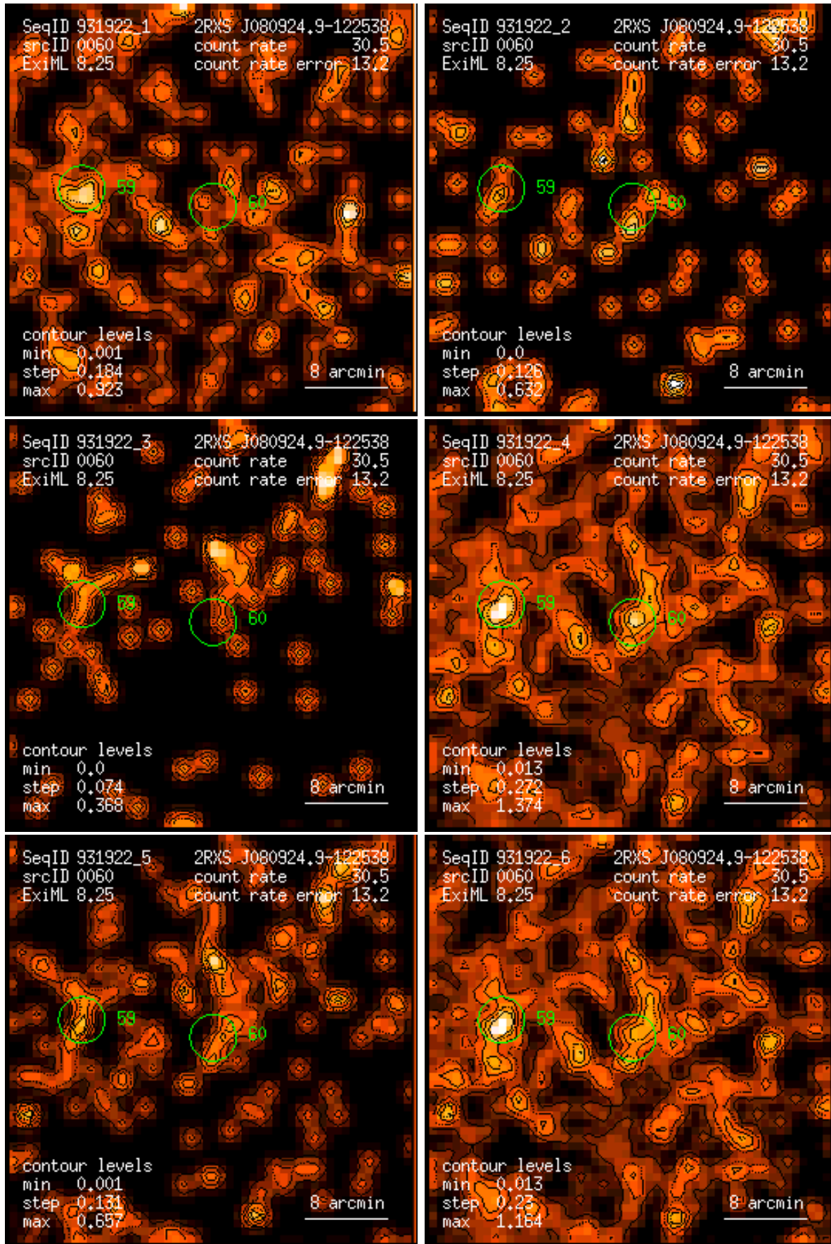
Figure 60: RASS 931922: detection 0060: band rate images, Gaussian filter: (1) PSPC channels 11 – 41, (2) 52 – 90, (3) 91 – 201, (4) 11 – 235, (5) 52 – 201, (6) 11 – 201. Broad band rates in counts/ks. Band rate contour levels in counts/ks/arcmin 2 .
