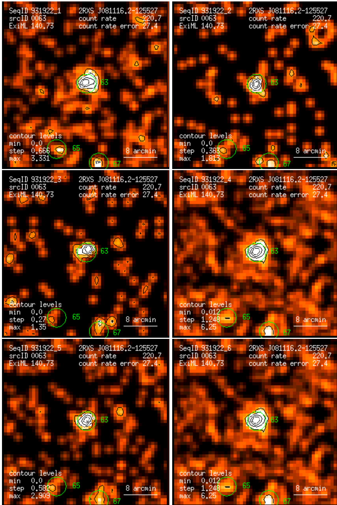
Figure 63: RASS 931922: detection 0063: band rate images, Gaussian filter: (1) PSPC channels 11 – 41, (2) 52 – 90, (3) 91 – 201, (4) 11 – 235, (5) 52 – 201, (6) 11 – 201. Broad band rates in counts/ks. Band rate contour levels in counts/ks/arcmin 2 .
